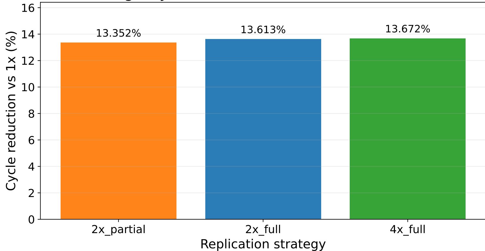
Average Cycle Reduction Across Cases 1 and 2
