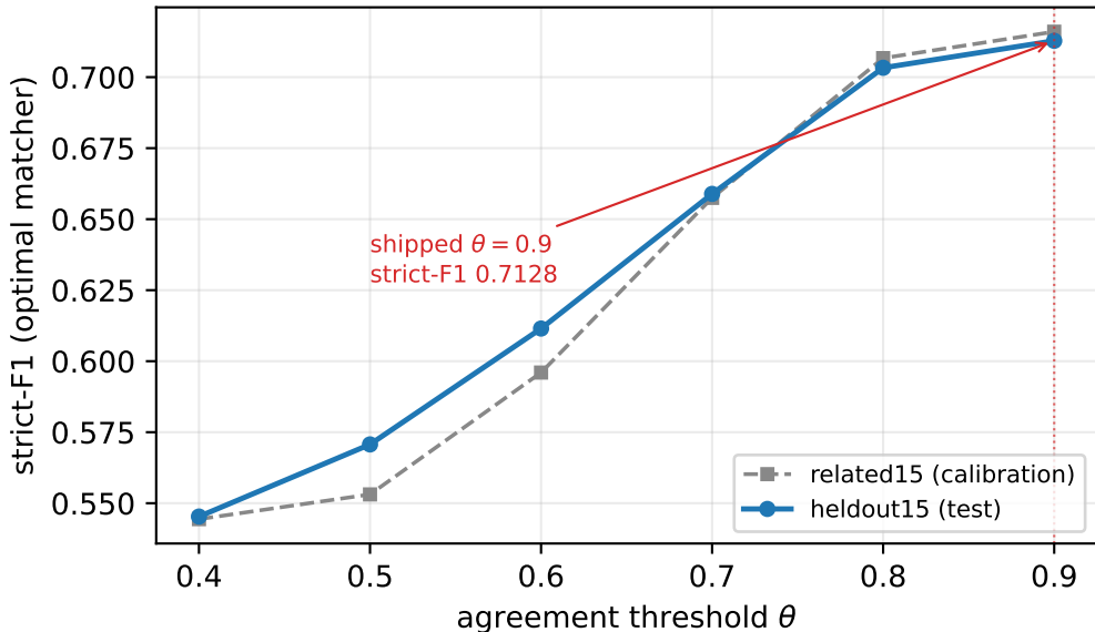
Held-out \theta -sweep vs calibration (at \theta_{\text{reject}} = 0.2 )
