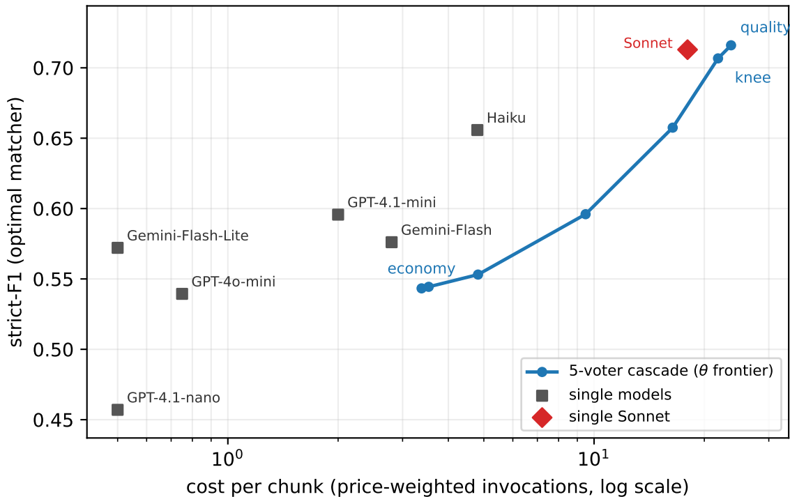
Cost--quality plane: 5-voter cascade frontier vs single models
