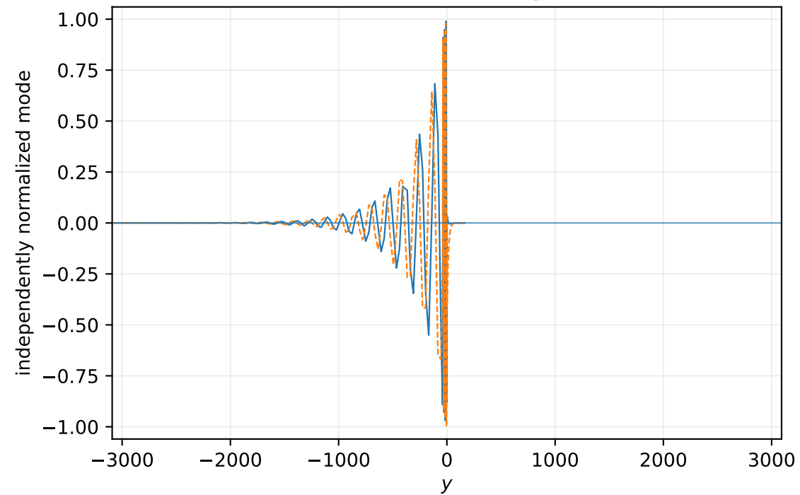
Transverse velocity \hat{v}
