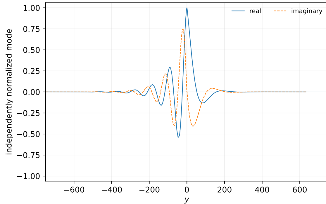
Streamwise velocity \hat{u}
