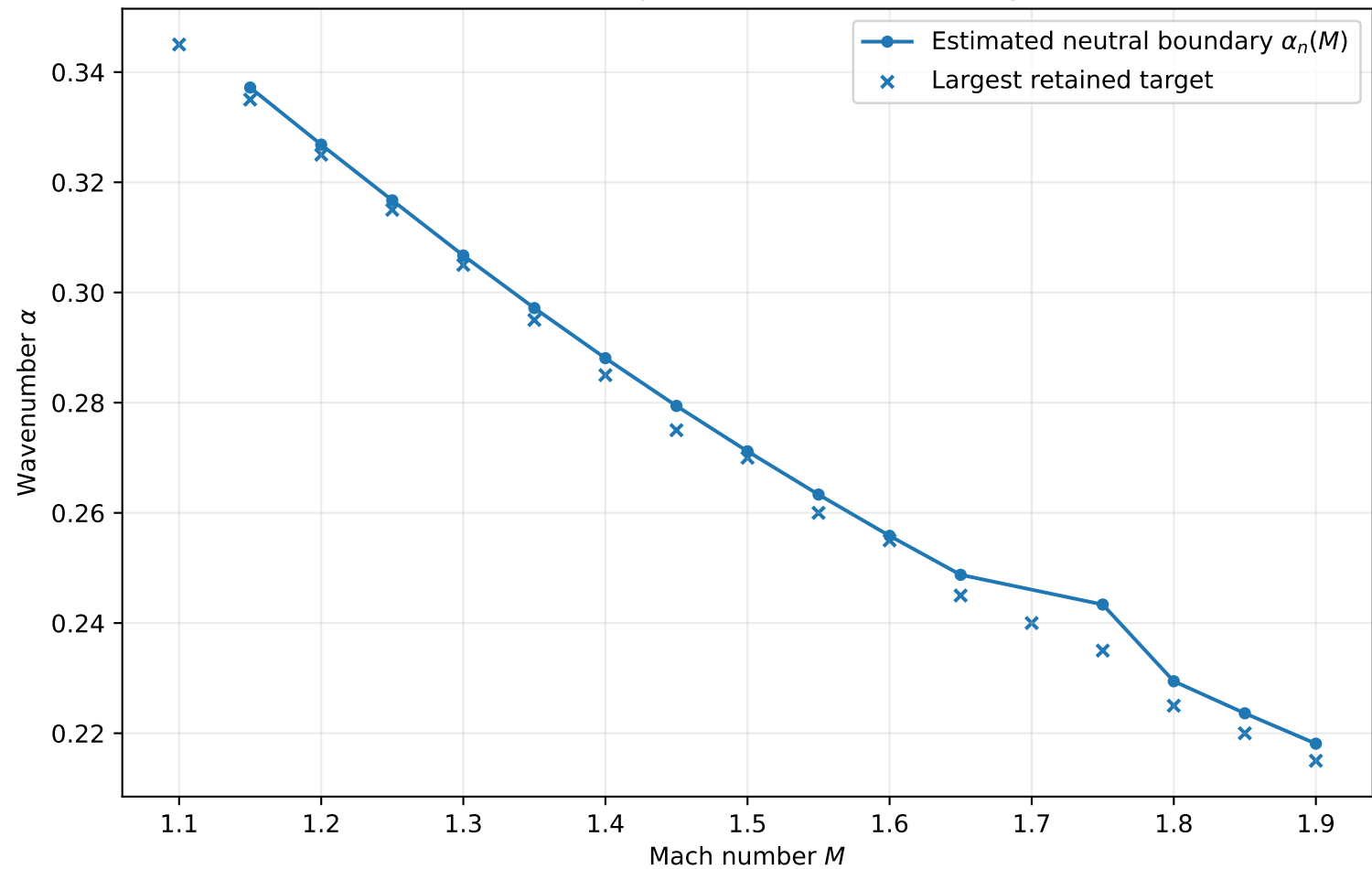
Classical supersonic neutral boundary
