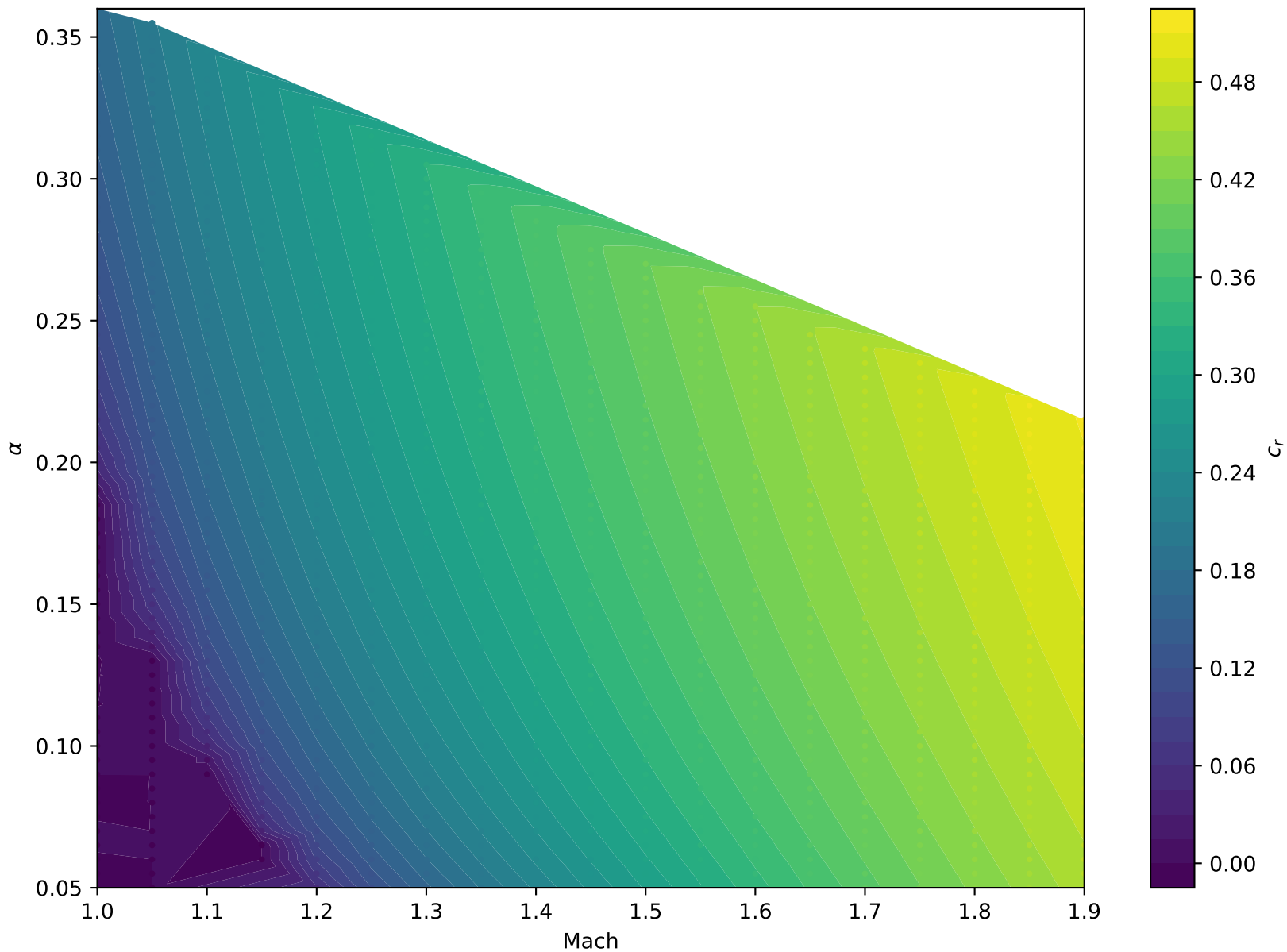
Classical supersonic dense reference: c_r(M, \alpha)
