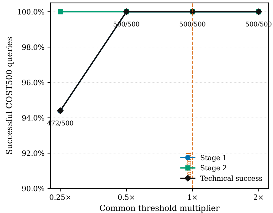
(a) Common scaling of both convergence thresholds
