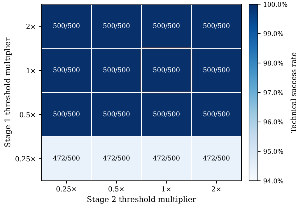
(b) Independent Stage 1 / Stage 2 sensitivity
