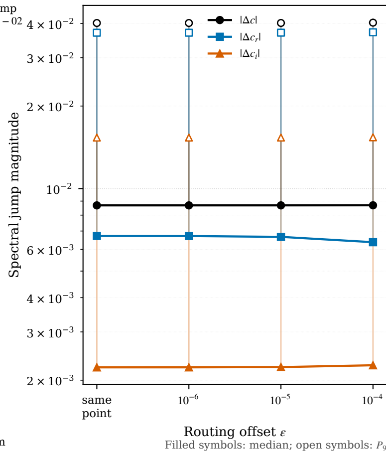
(b) Routed jump as \varepsilon \rightarrow 0
