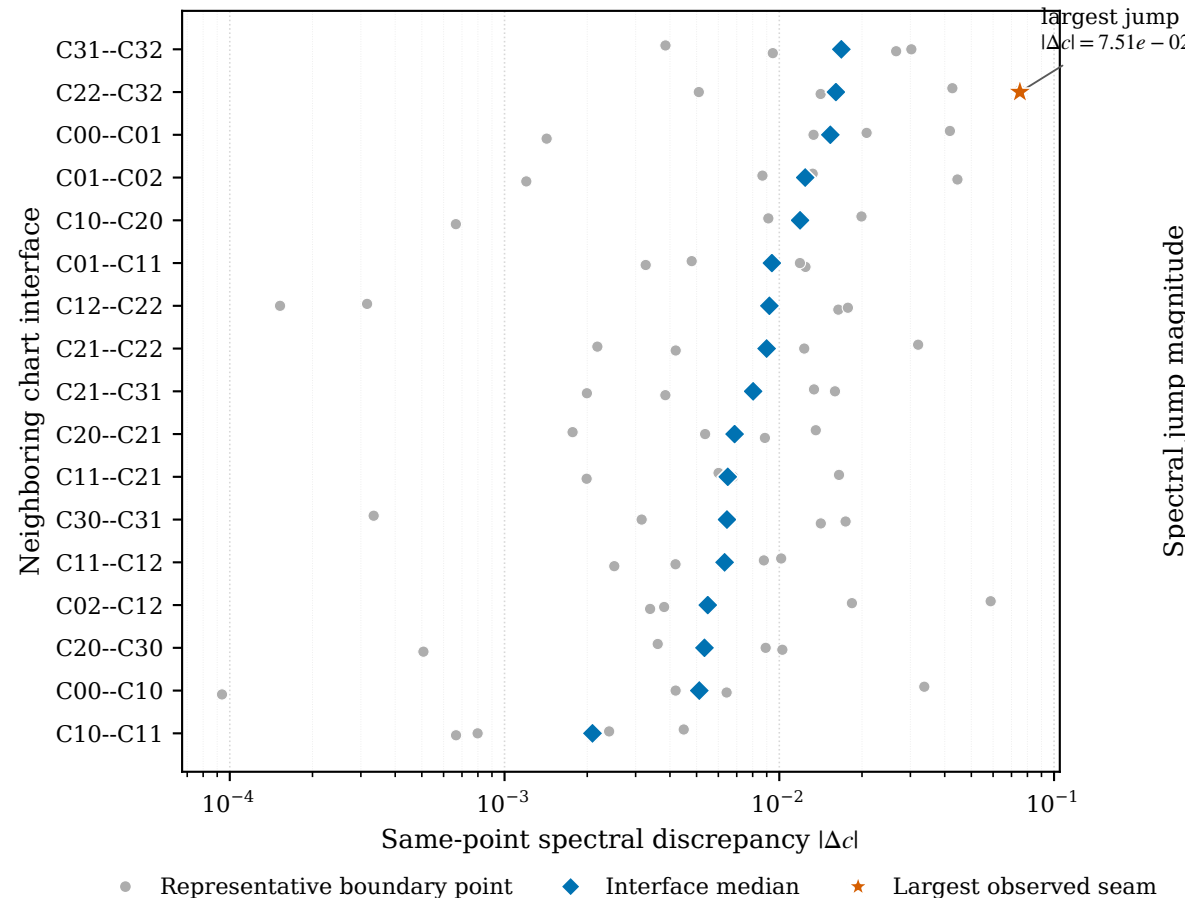
(a) Same-point discontinuities across routing interfaces
