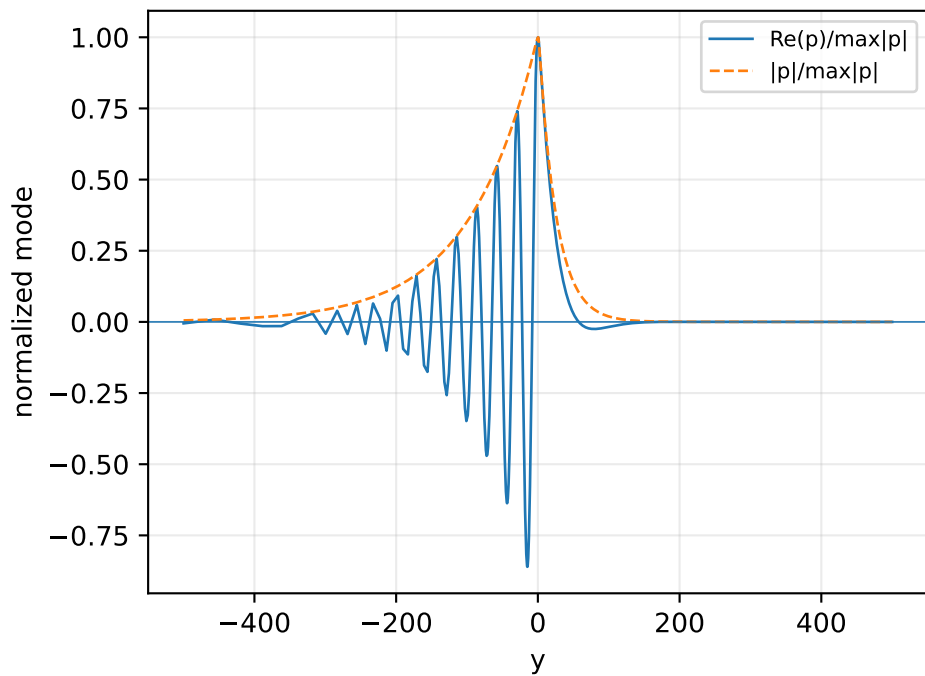
M=1.50, alpha=0.15000 ci=0.041824, N=4594
