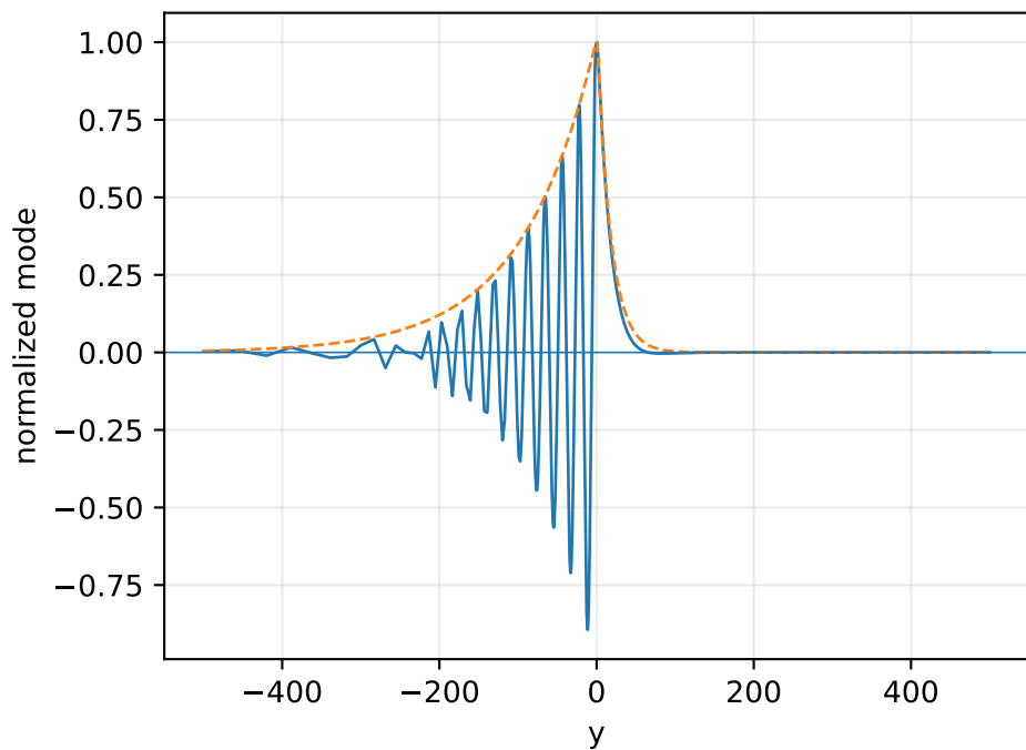
M=1.50, alpha=0.16250 ci=0.038006, N=4594
