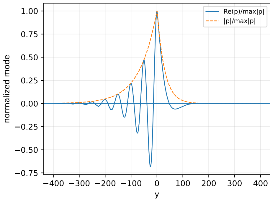
M=1.30, alpha=0.15000 ci=0.069919, N=4594
