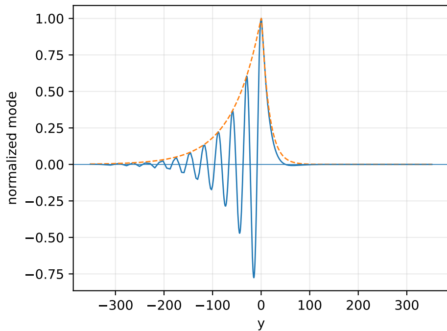
M=1.30, alpha=0.18333 ci=0.055355, N=4594
