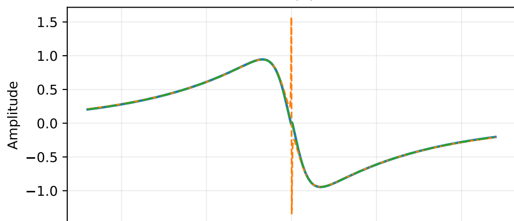
Re ( u )
