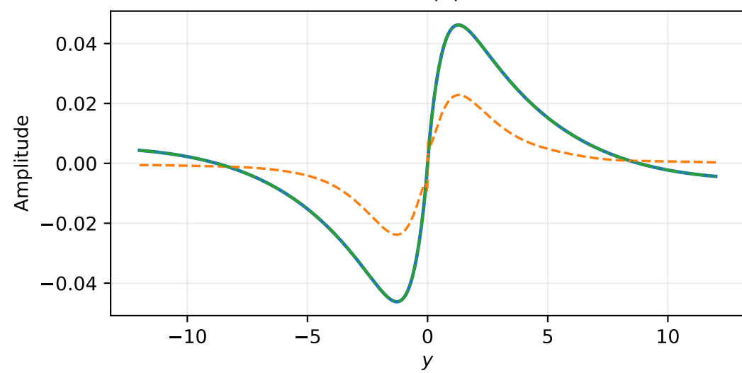
Re ( v )
