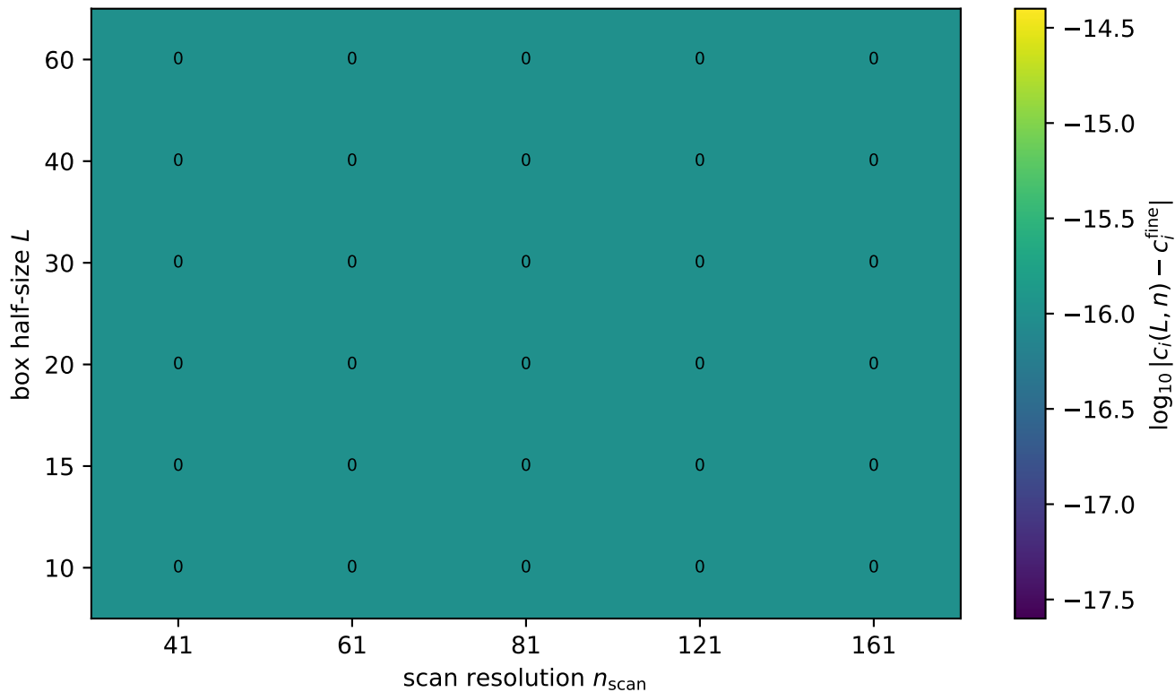
Subsonic classical convergence, \alpha = 0.5 , M = 0.5
