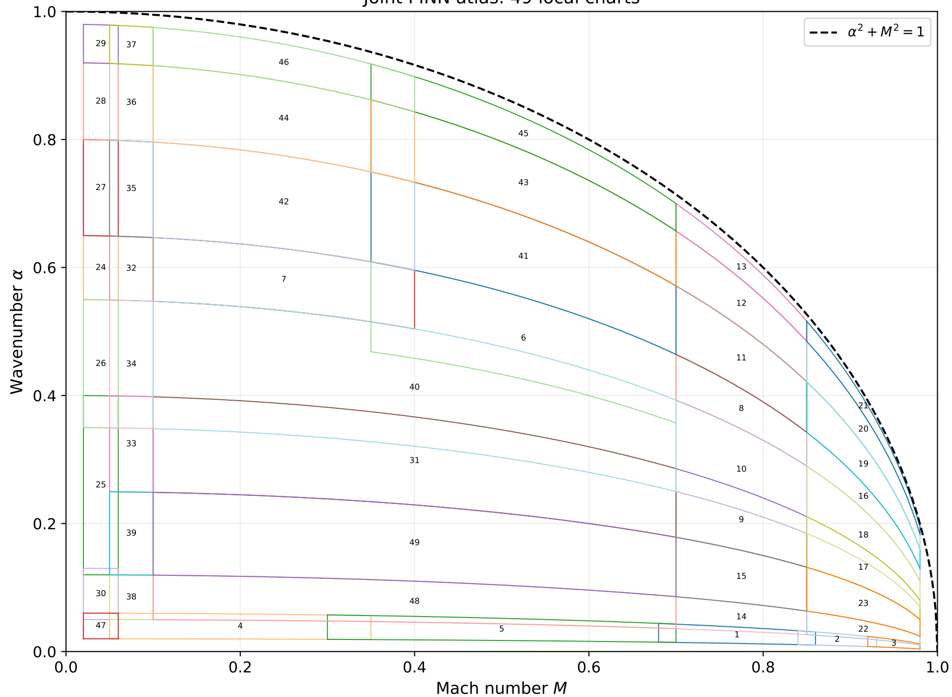
Joint PINN atlas: 49 local charts
