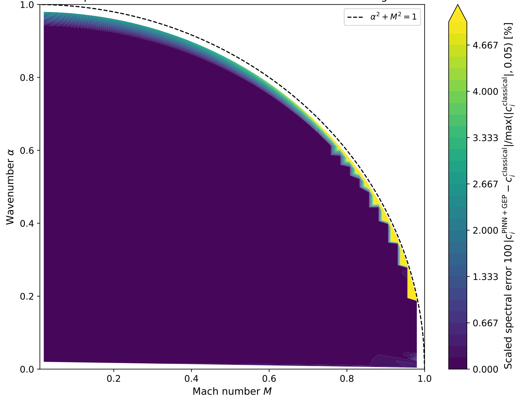
Spectral error: N340 PINN + GEP versus classical shooting
