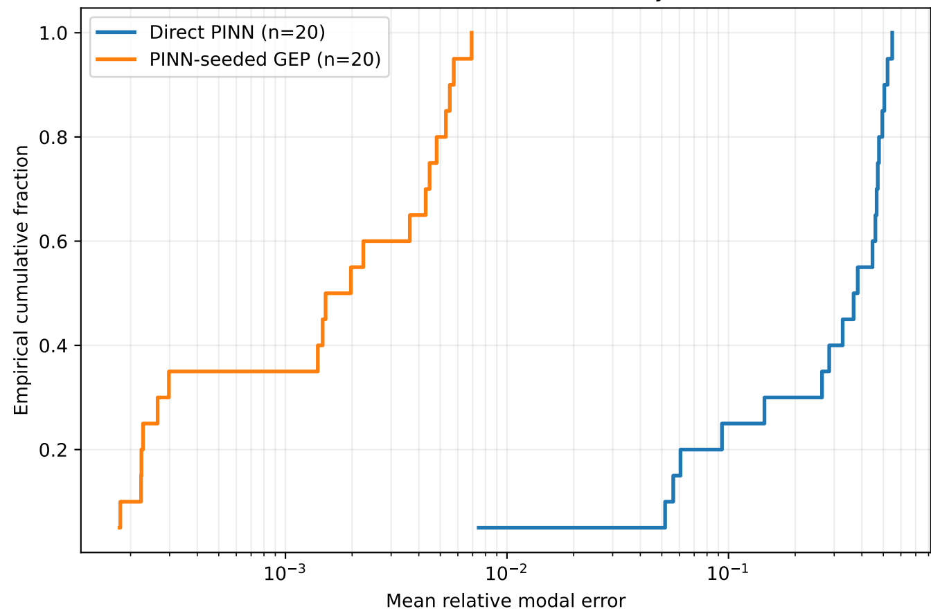
Paired modal reconstruction accuracy — N340
