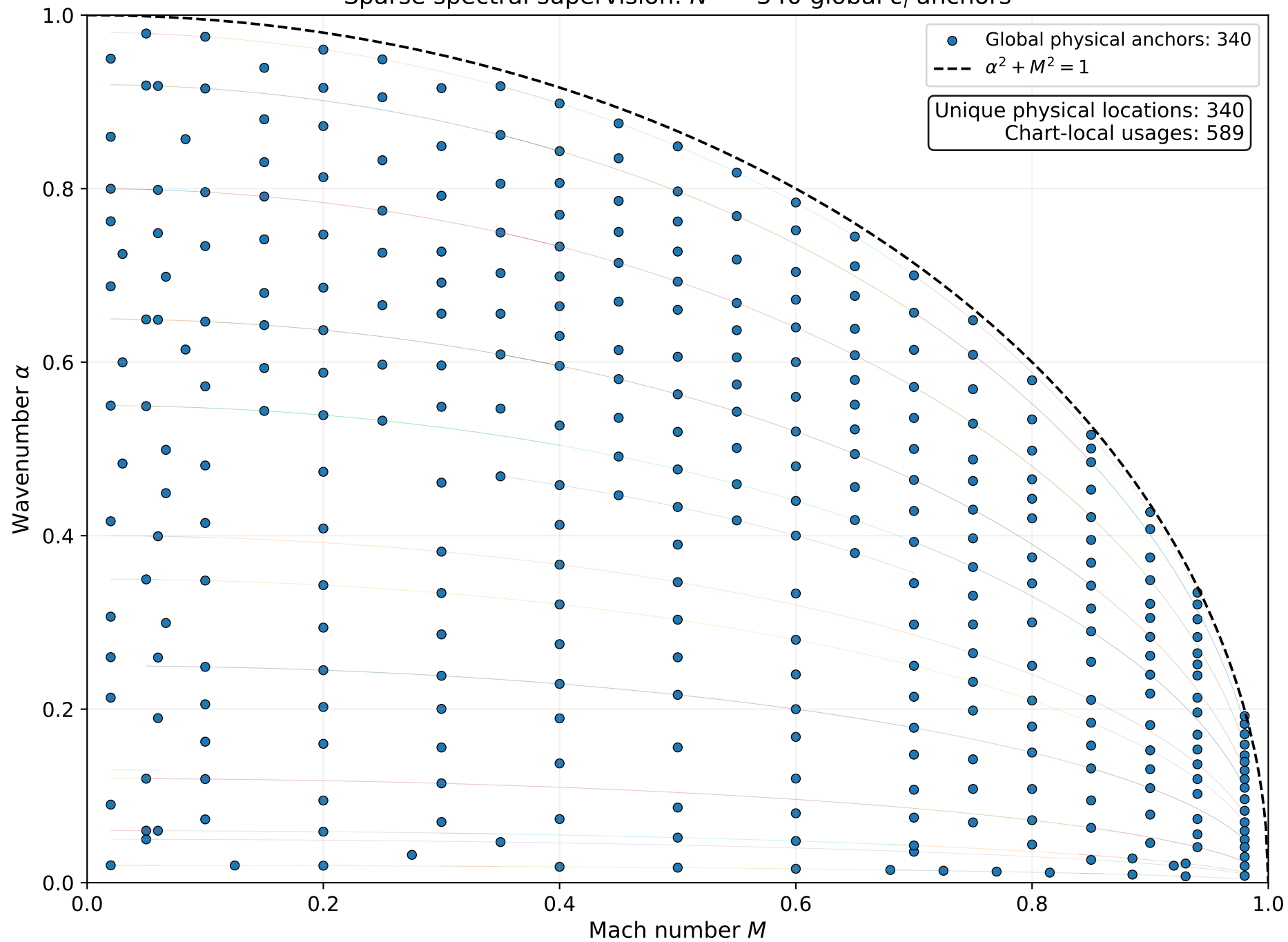
Sparse spectral supervision: N^* = 340 global c_i anchors
