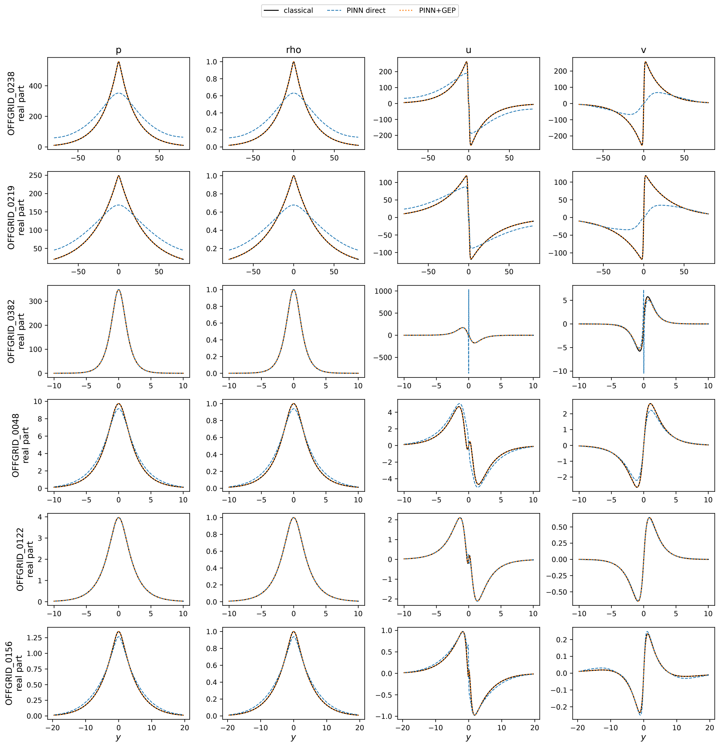
Representative modal profiles: classical, direct PINN and PINN-seeded GEP
