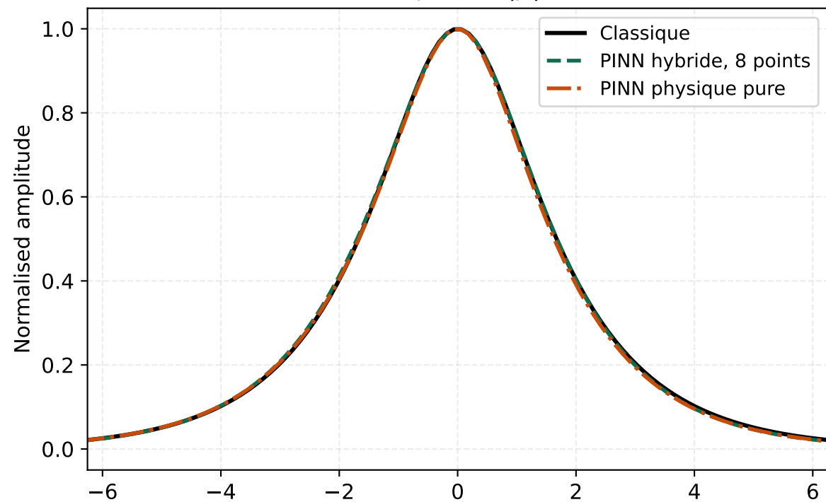
Amplitude |\hat{p}|
