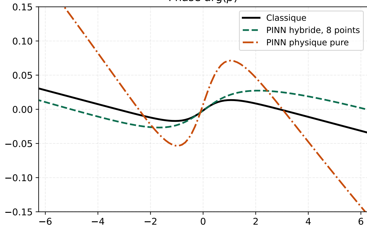
Phase \arg(\hat{p})
