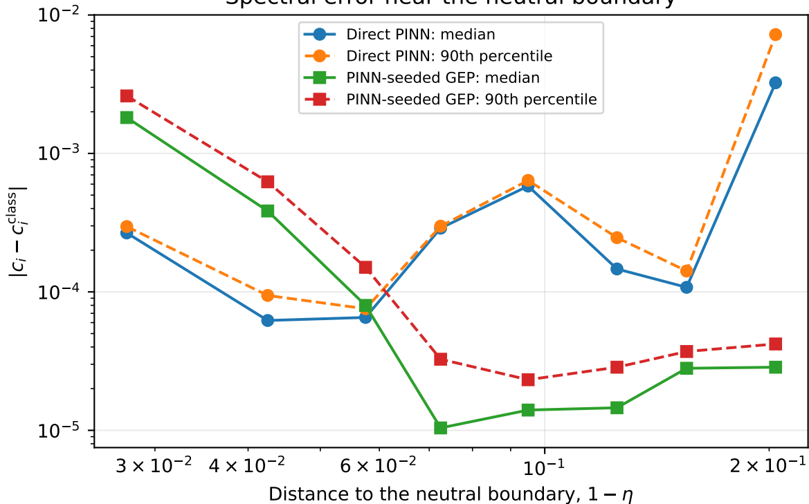
Spectral error near the neutral boundary
