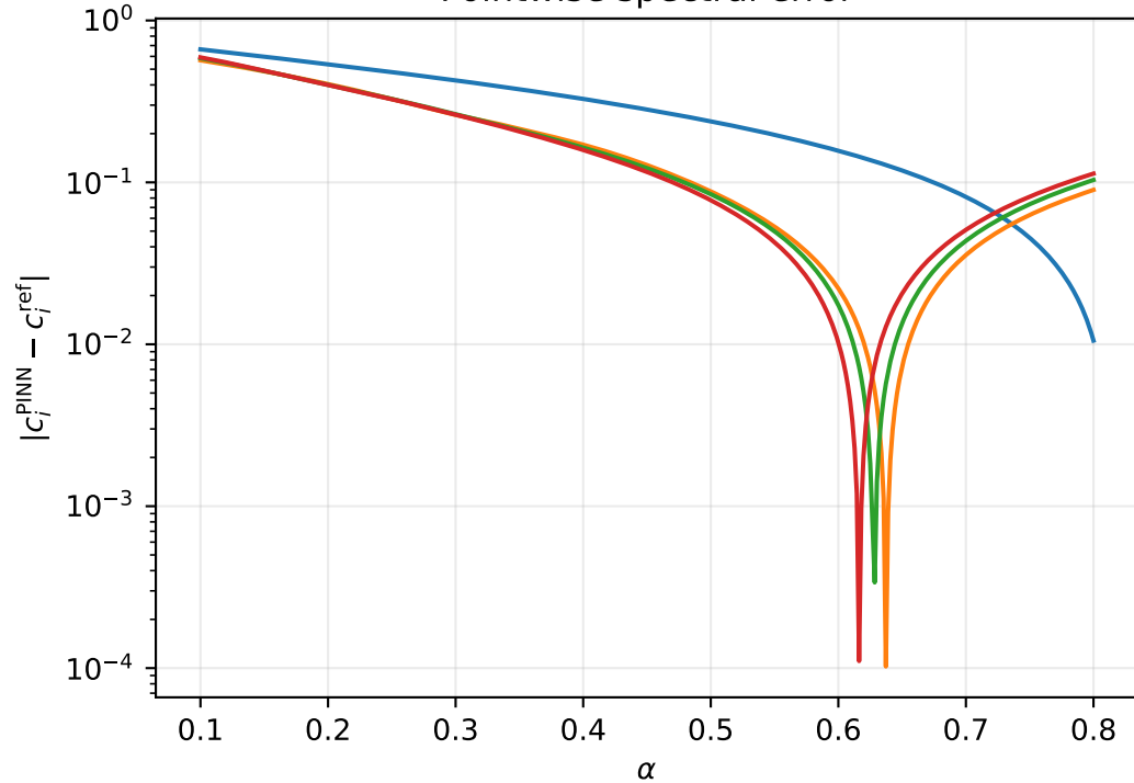
Pointwise spectral error
