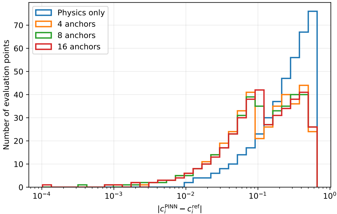
Distribution of spectral errors
