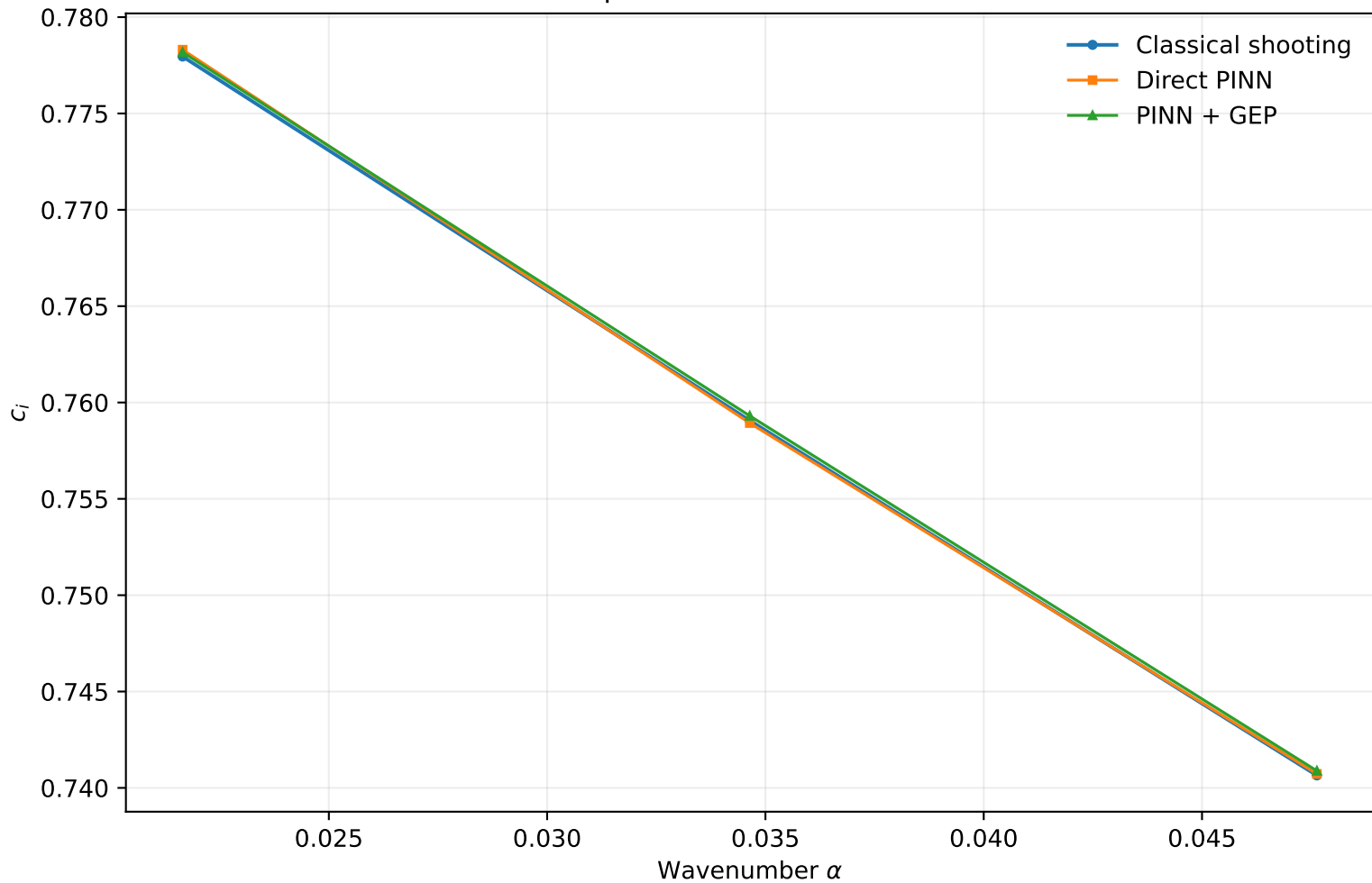
Spectral cut at M = 0.5
