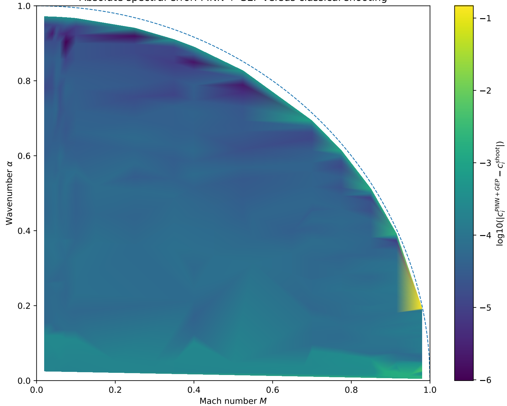
Absolute spectral error: PINN + GEP versus classical shooting
