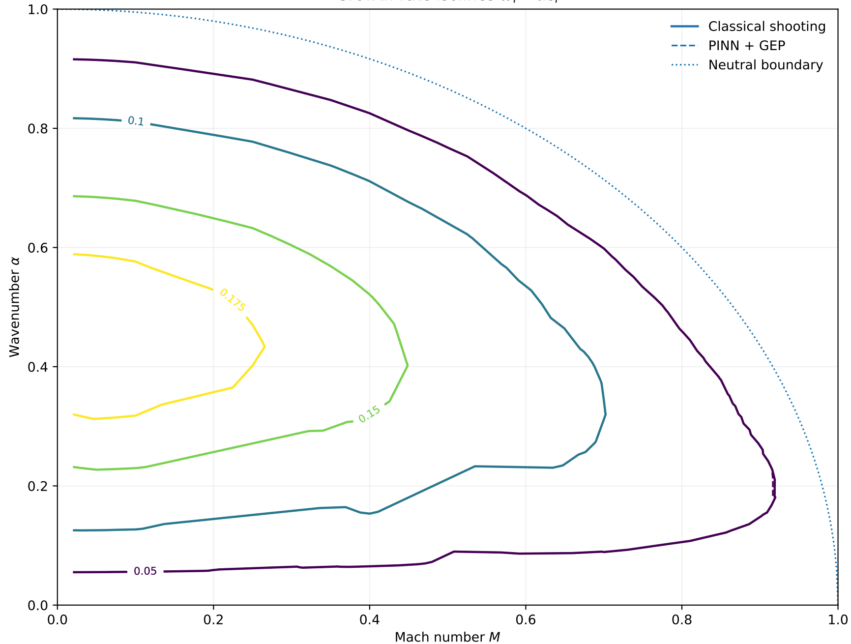
Growth-rate isolines \omega_i = \alpha c_i
