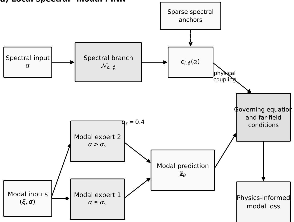
(a) Local spectral--modal PINN
