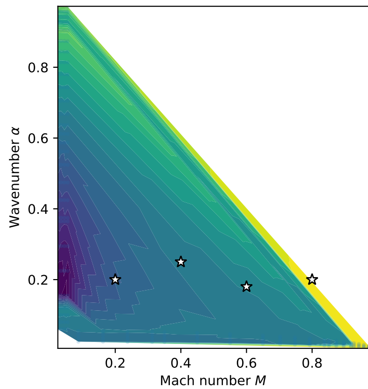
PINN-seeded GEP: u
