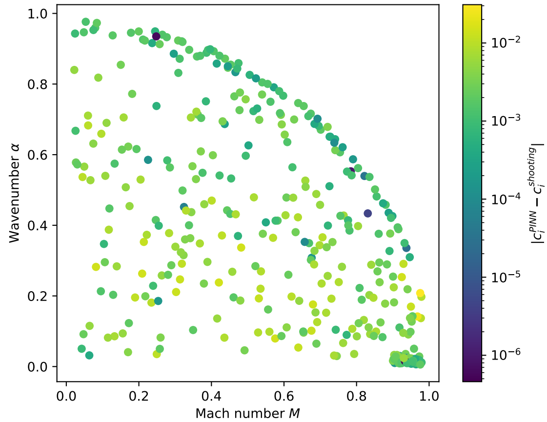
Pointwise direct-PINN error
