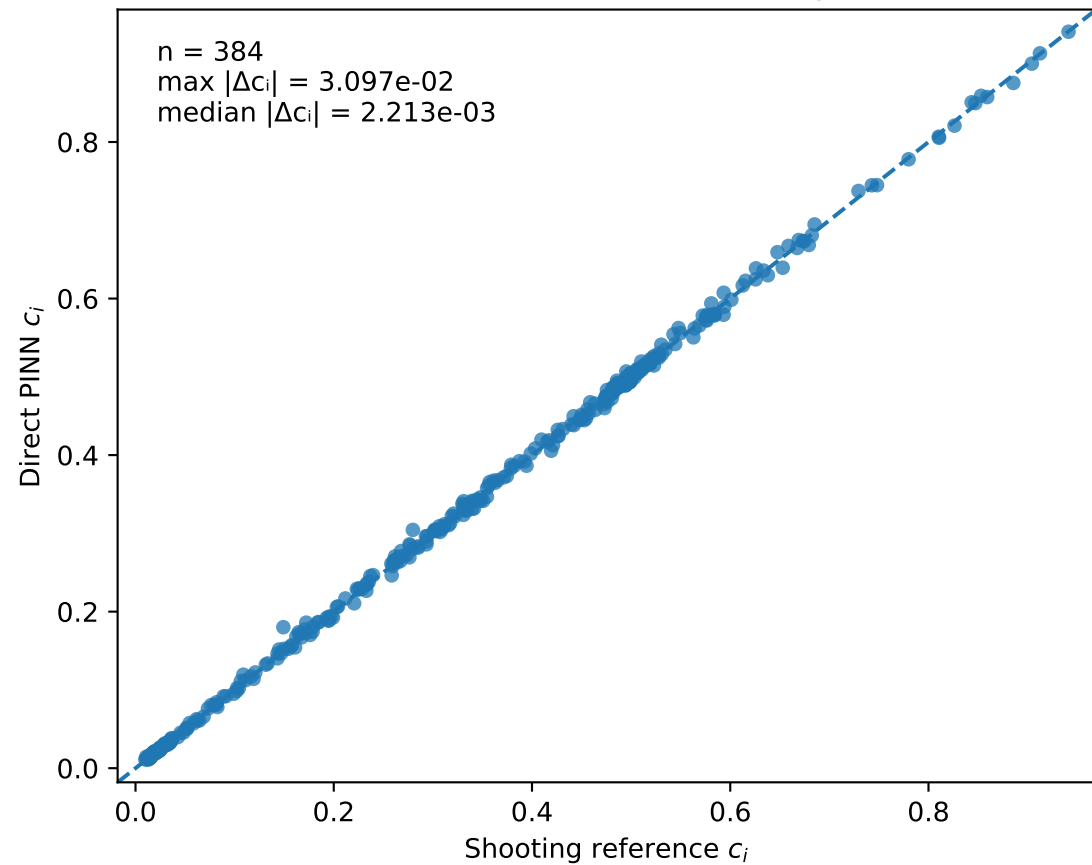
Direct PINN versus shooting
