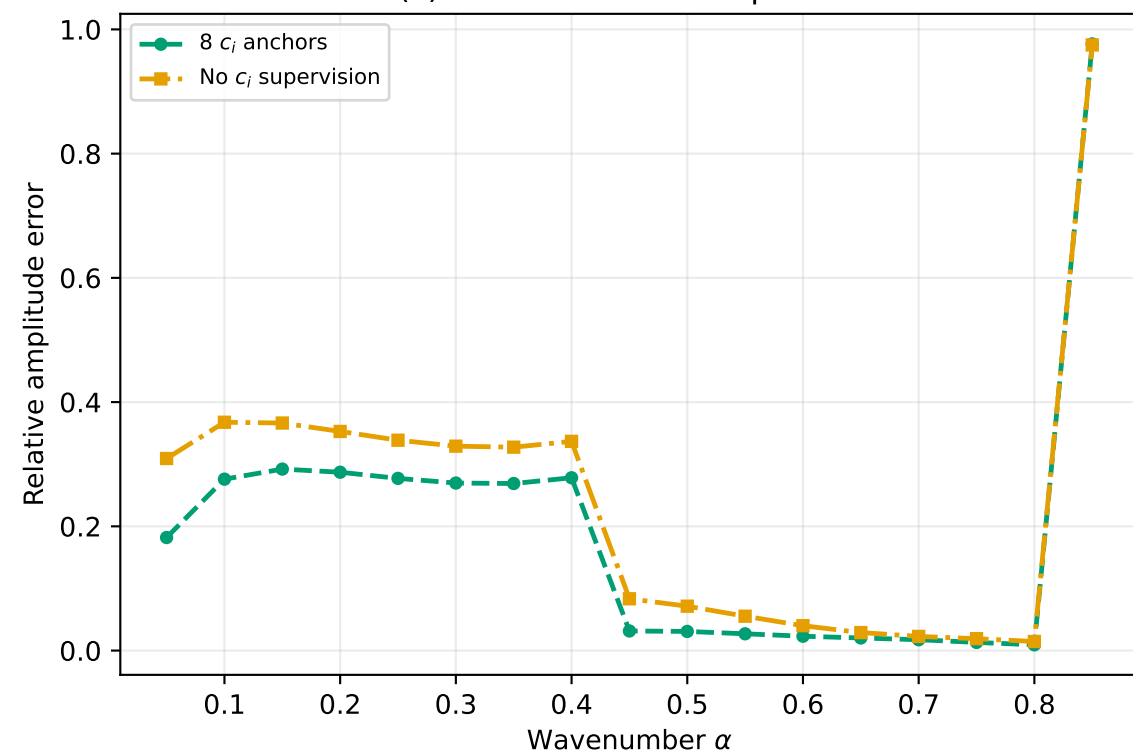
(c) Pressure-mode amplitude
