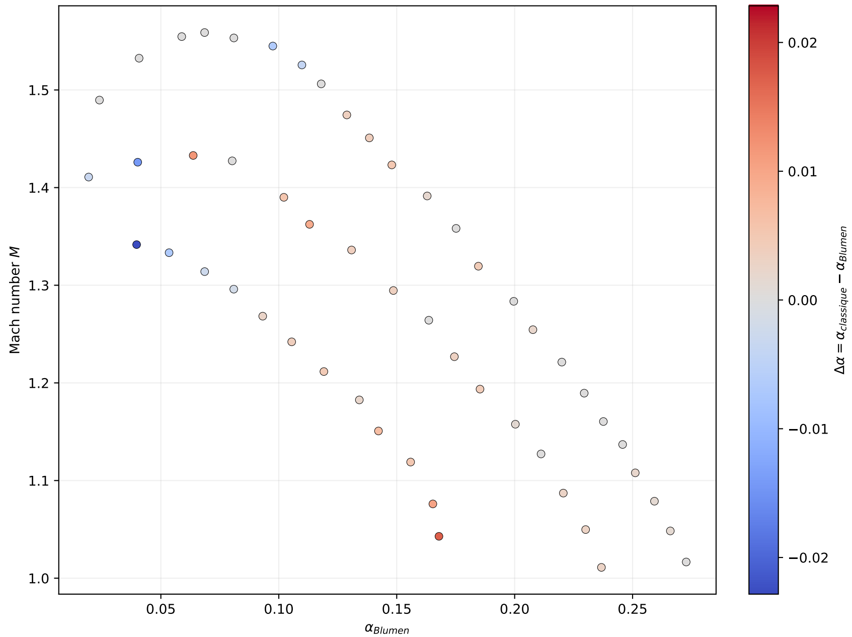
Geometric error of the Blumen isolines
