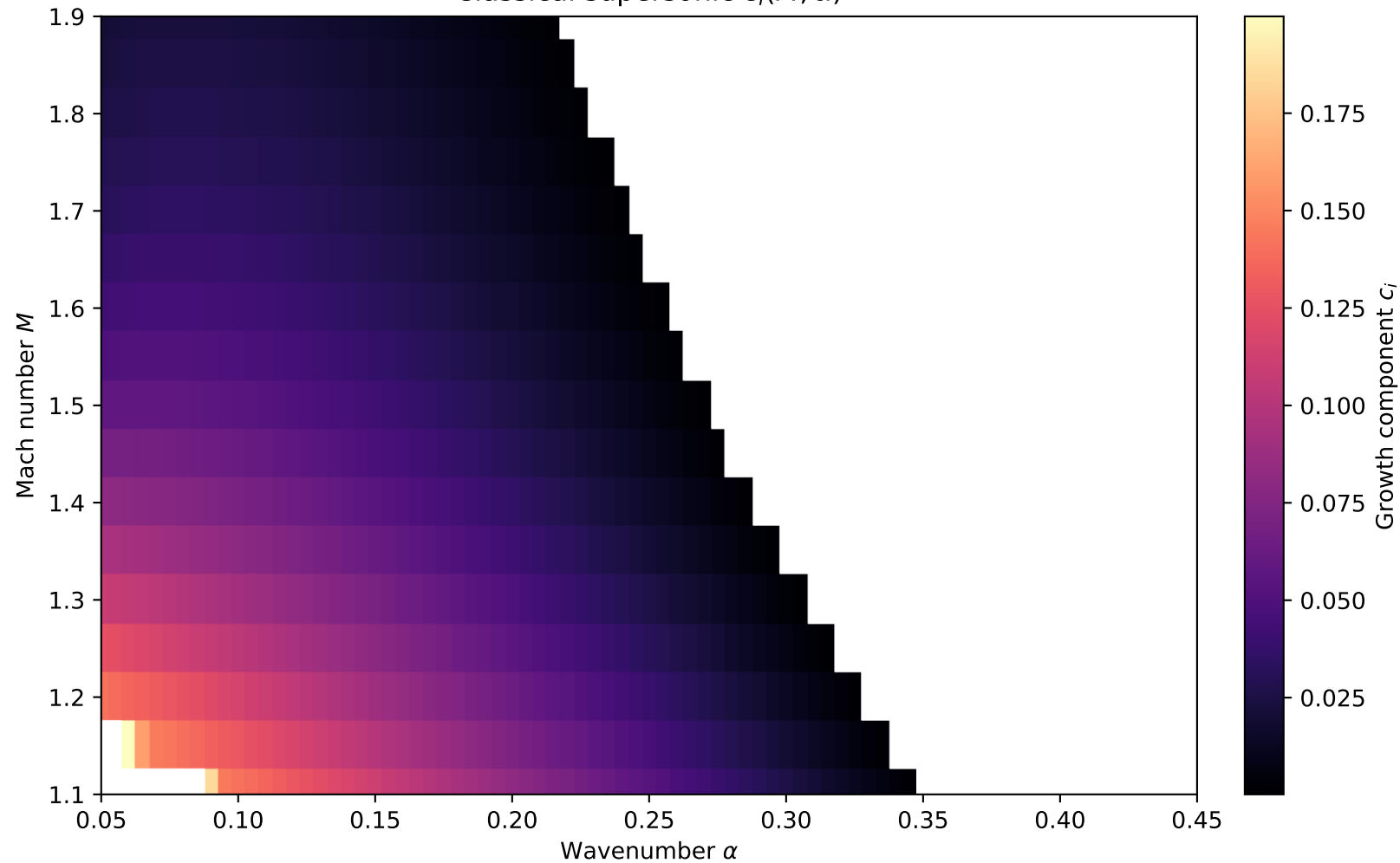
Classical supersonic c_i(M, \alpha)
