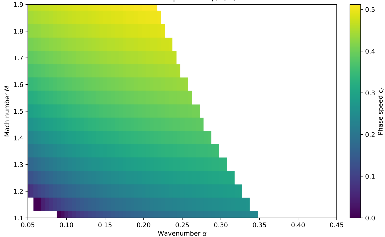
Classical supersonic c_r(M, \alpha)
