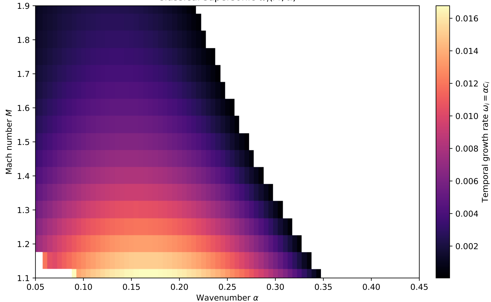
Classical supersonic \omega_i(M, \alpha)
