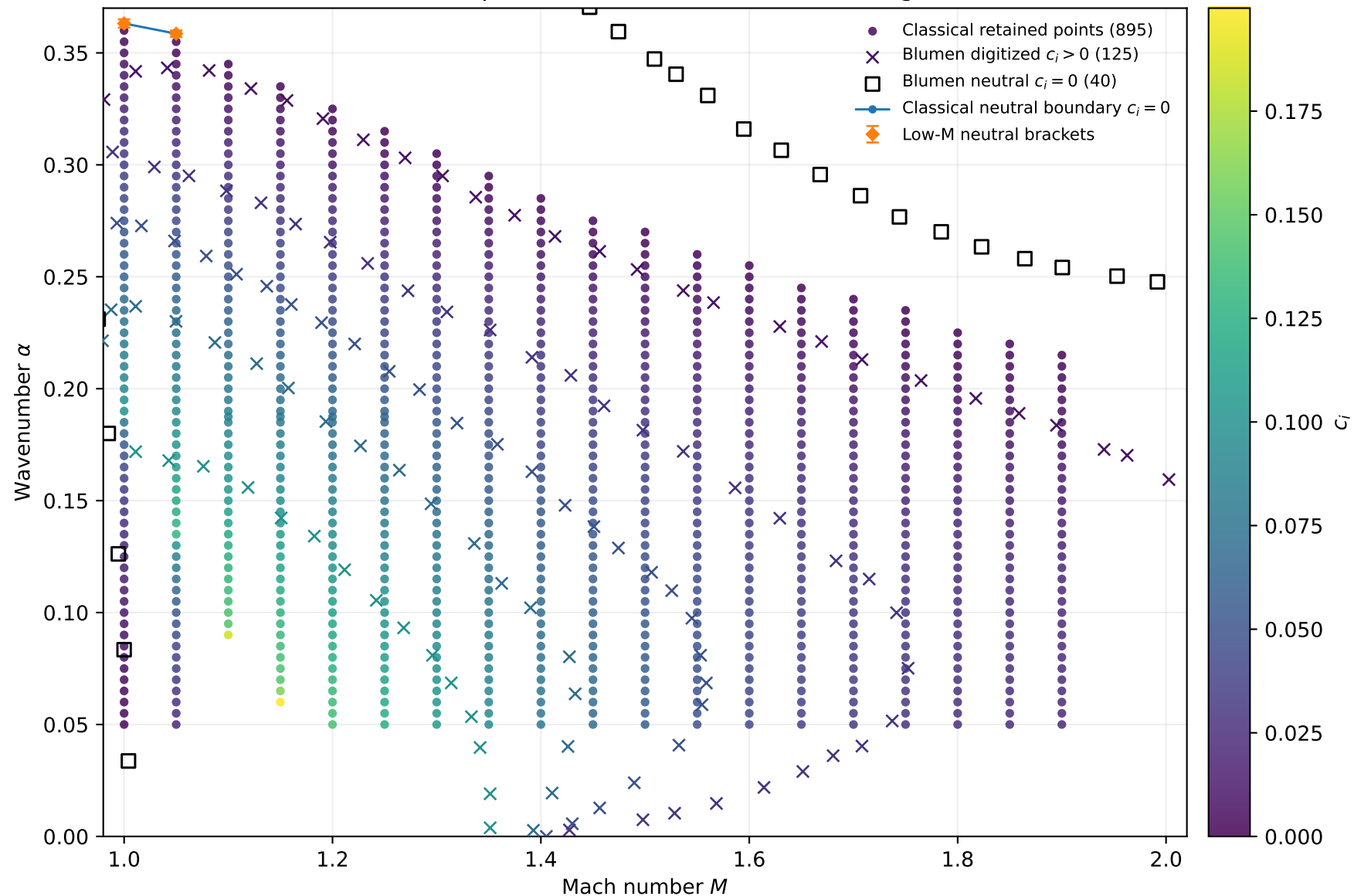
Final classical supersonic reference and Blumen digitization
