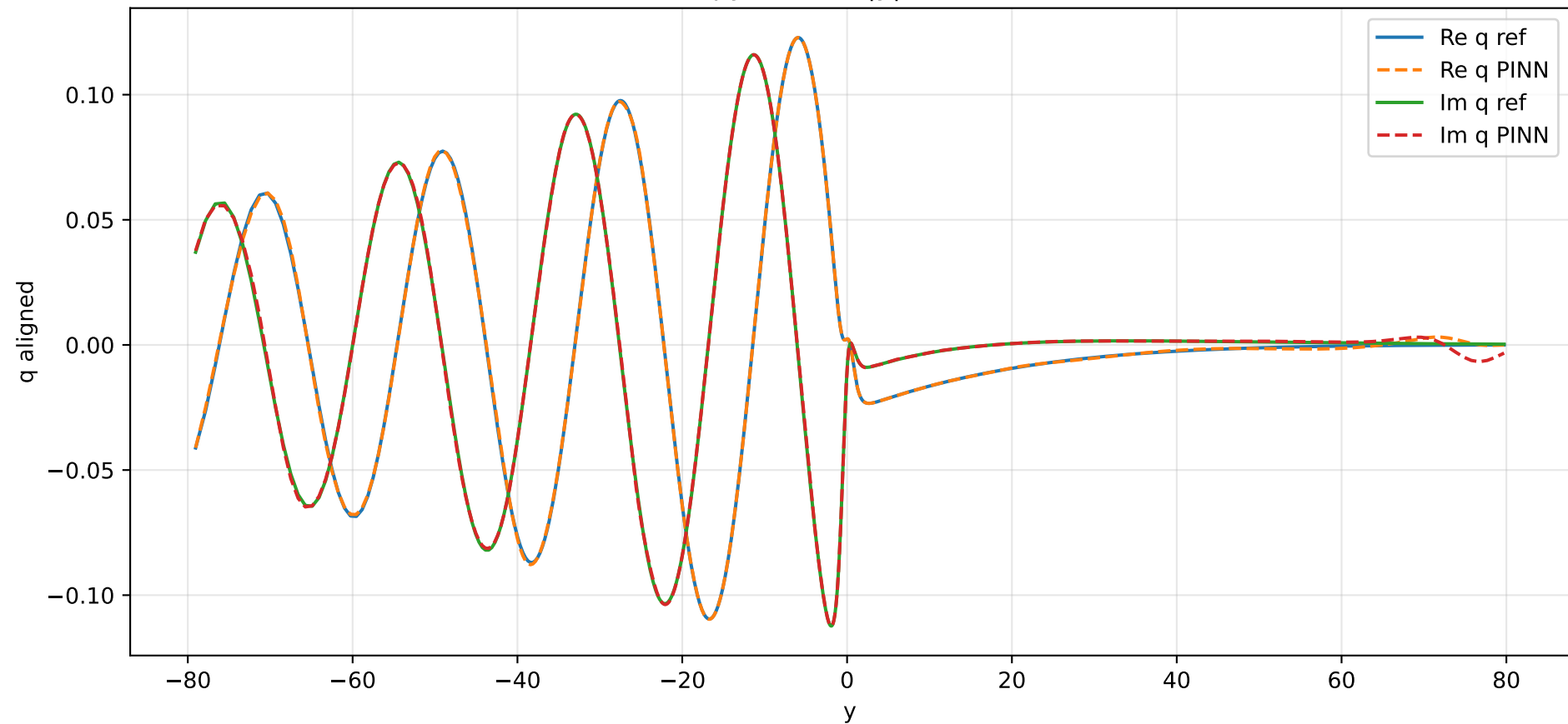
q(y) , centre |y| \leq 80
