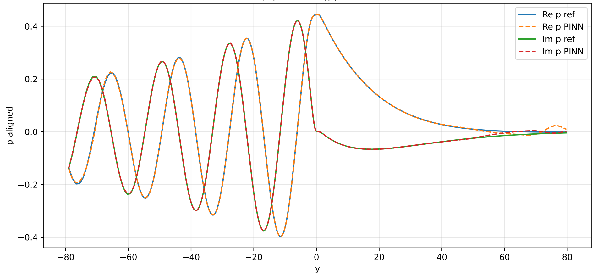
p(y) , centre |y| \leq 80
