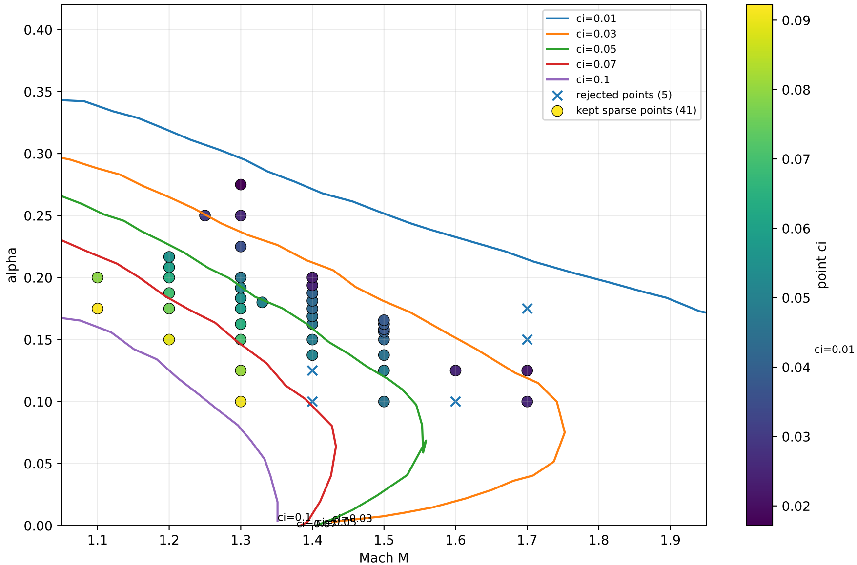
Supersonic sparse PINN points filtered on digitized Blumen ci isolines
