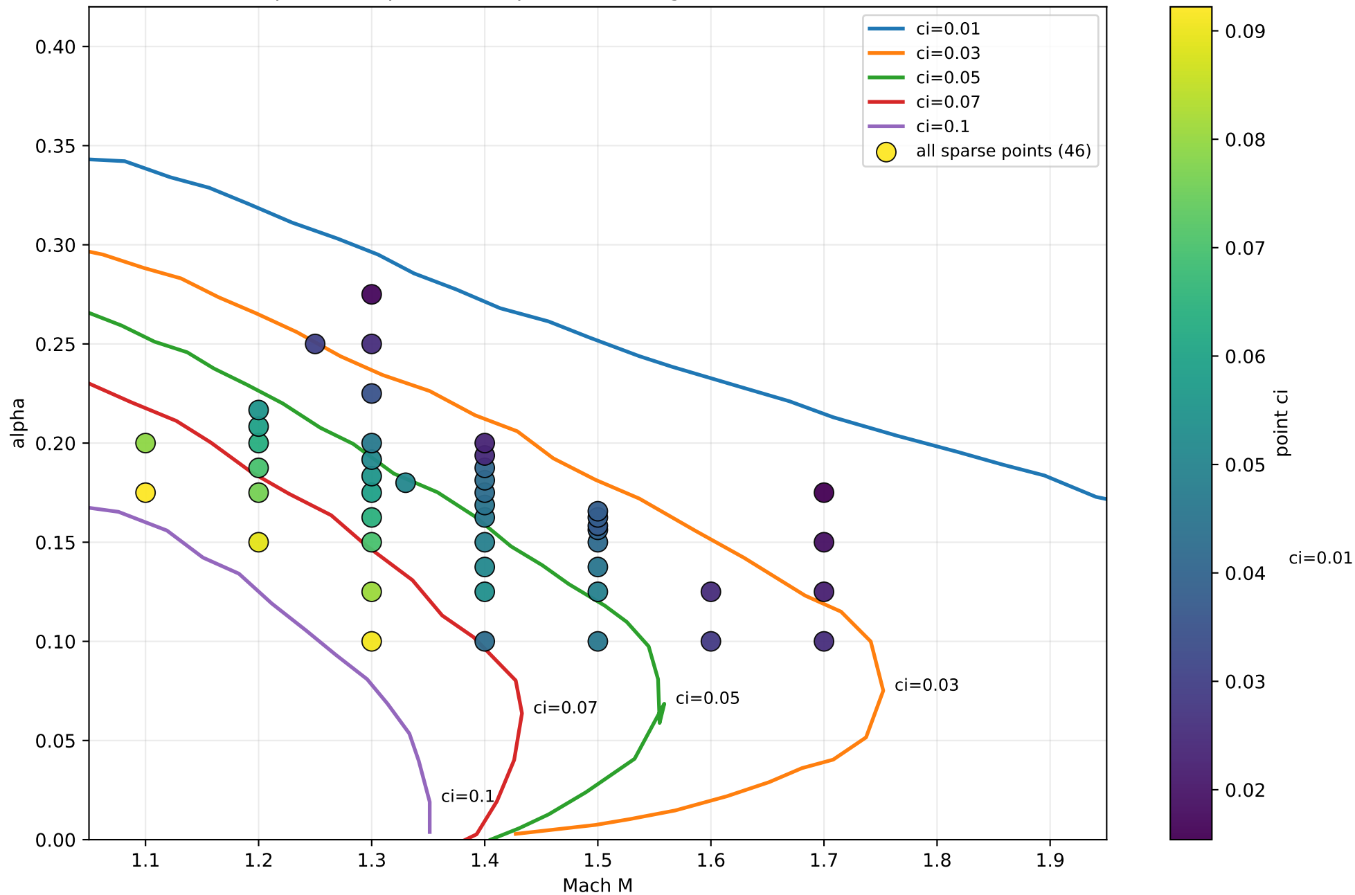
Supersonic sparse PINN points over digitized Blumen ci isolines
