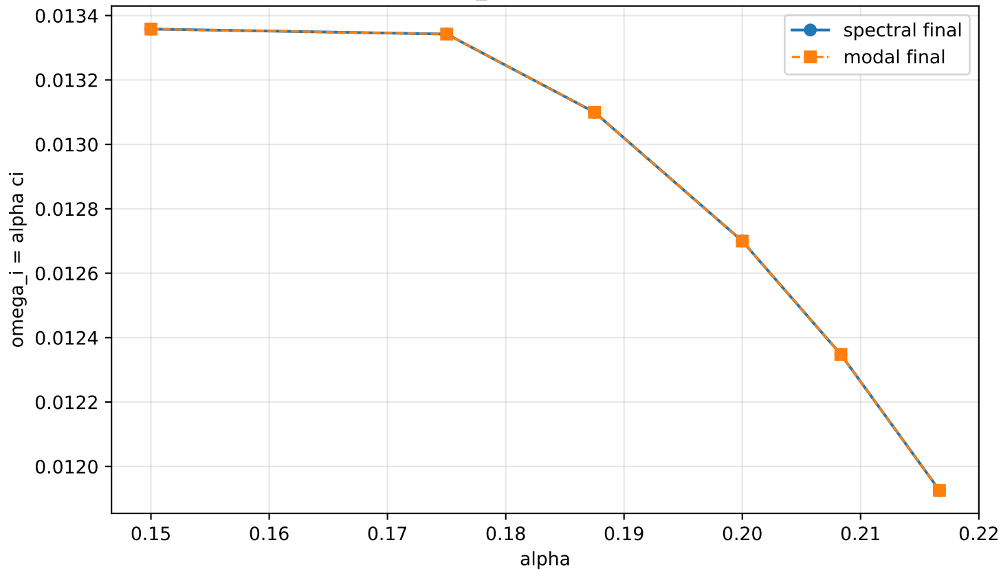
Final23 \omega_i = \alpha \text{ci}(\alpha) , M=1.2
