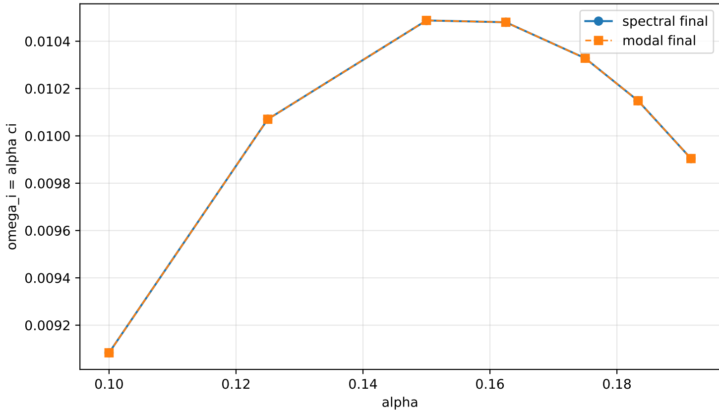
Final23 \omega_i = \alpha \text{ci}(\alpha) , M=1.3
