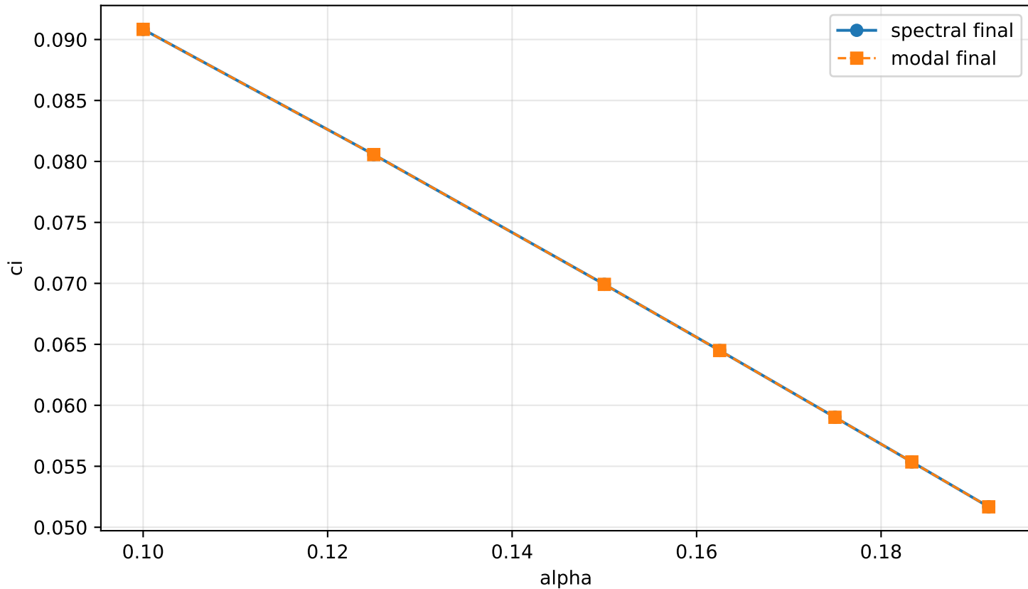
Final23 ci(alpha), M=1.3
