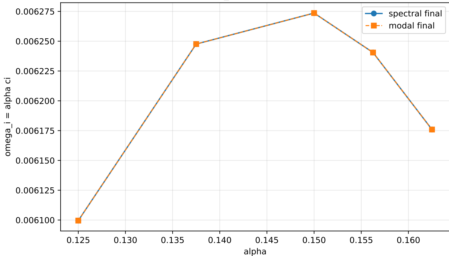
Final23 omega_i = alpha ci(alpha), M=1.5
