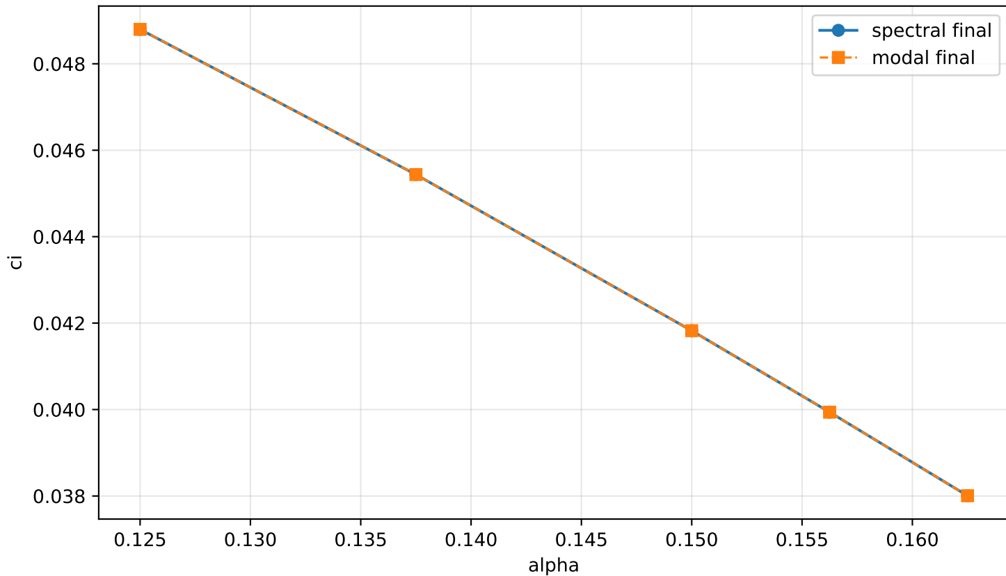
Final23 ci(alpha), M=1.5
