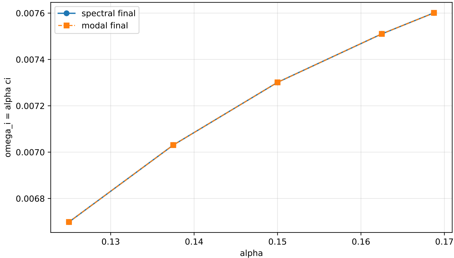
Final23 \omega_i = \alpha c_i(\alpha) , M=1.4
