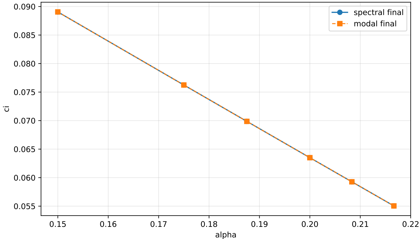
Final23 ci(alpha), M=1.2
