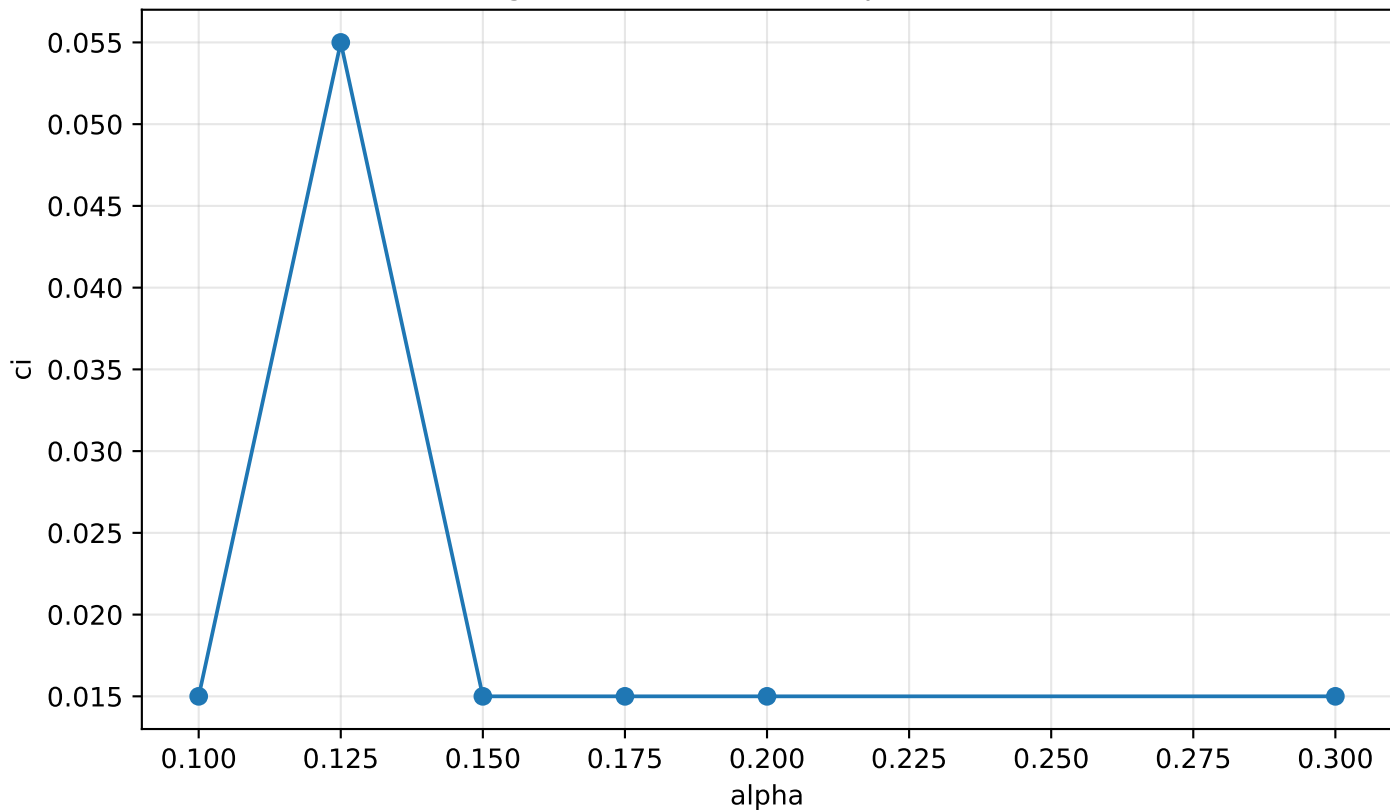
High Mach selected ci(alpha), M=1.6
