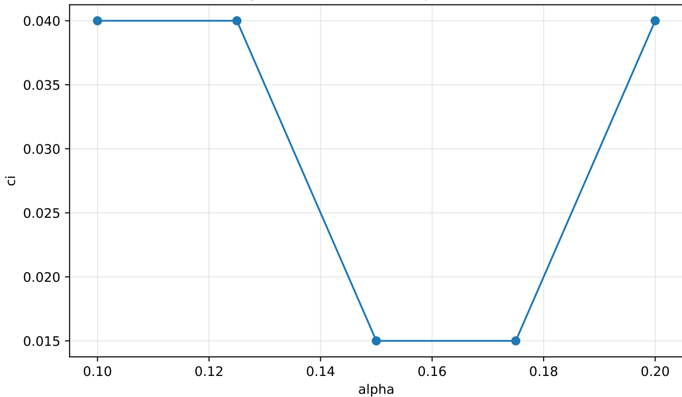
High Mach selected ci(alpha), M=1.8
