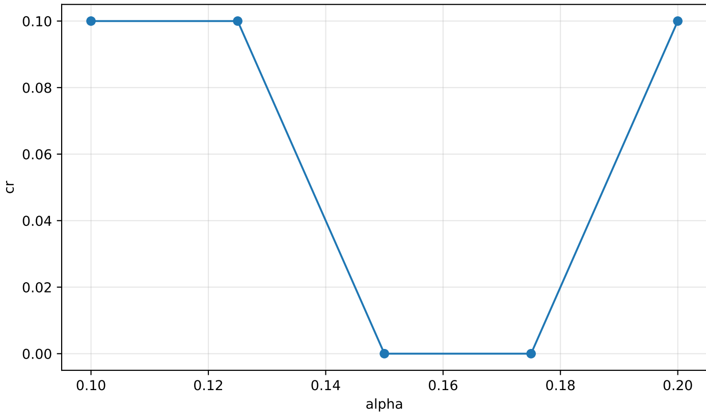
High Mach selected cr(alpha), M=1.8
