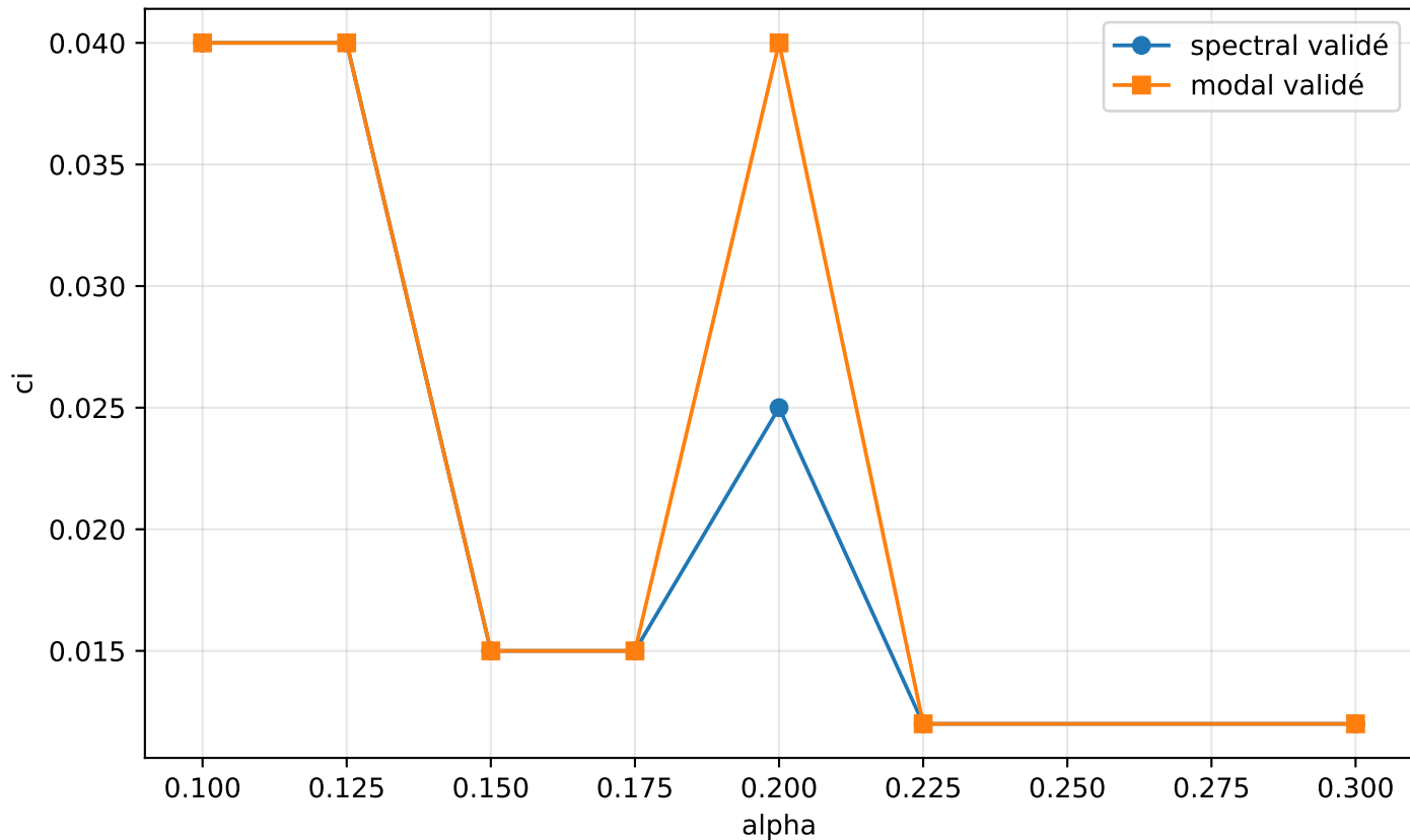
Supersonic ci(alpha), M=1.8
