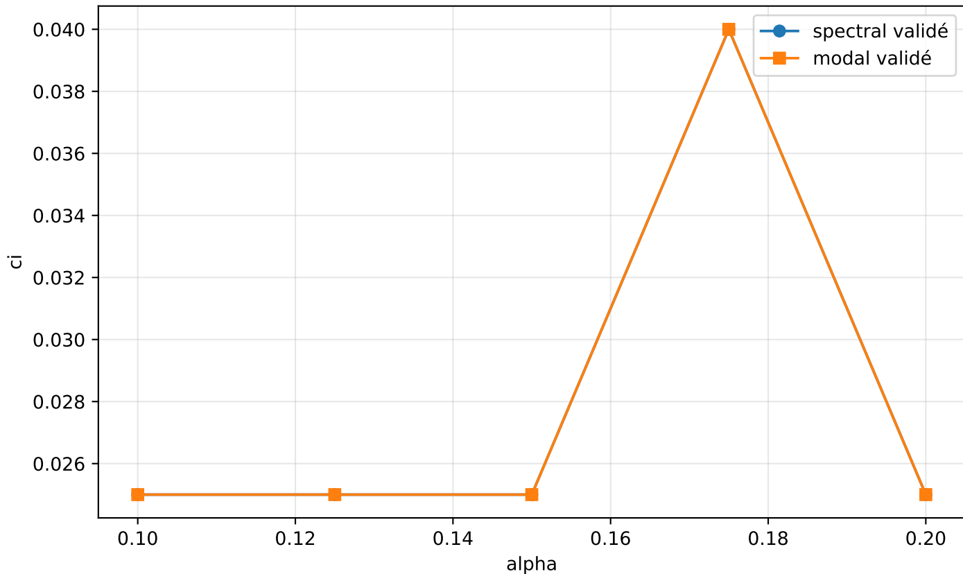
Supersonic ci(\alpha) , M=1.7
