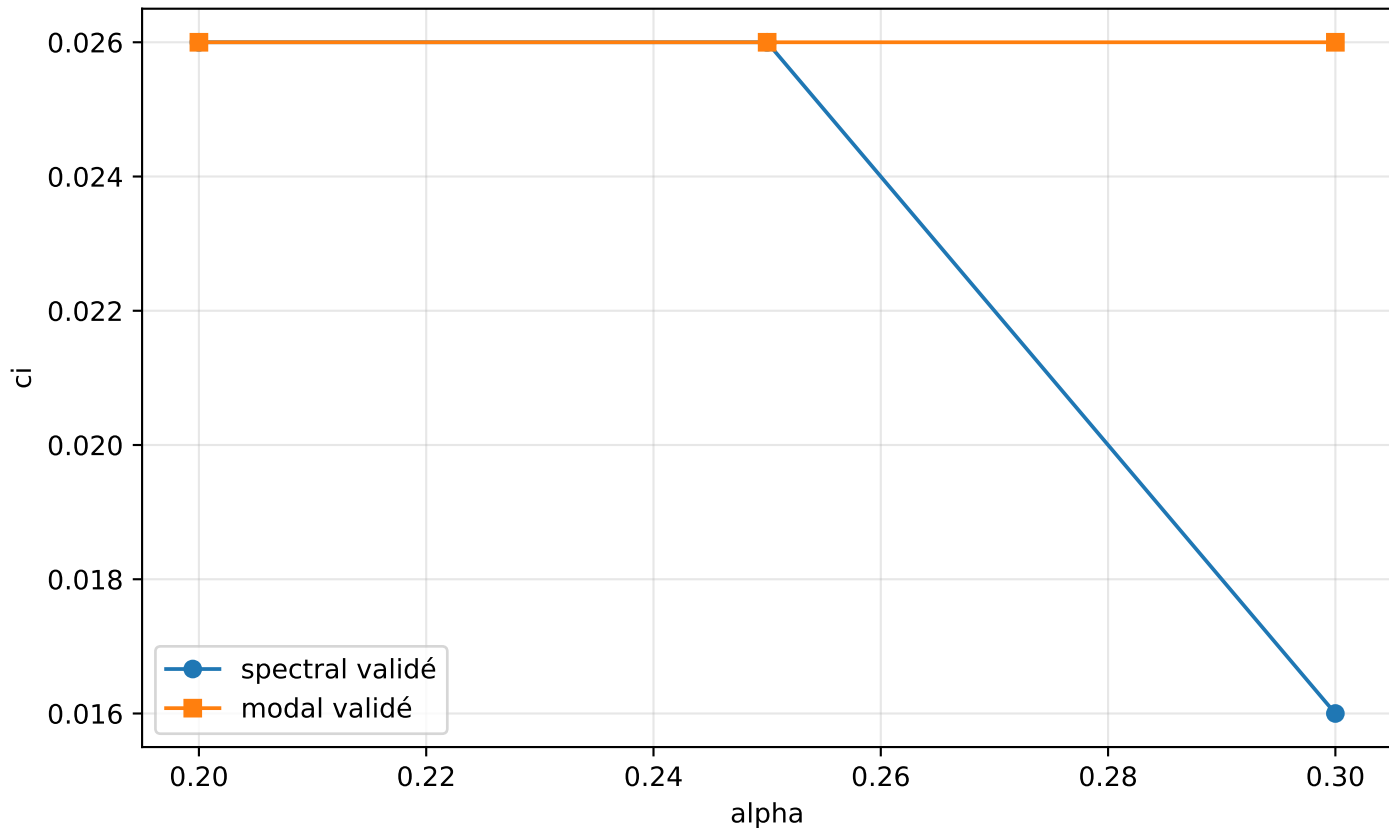
Supersonic c_i(\alpha) , M=1.9
