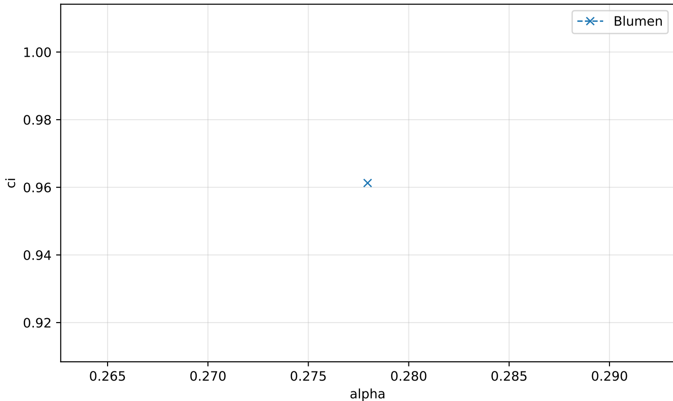
Supersonic c_i(\alpha) , M=0.277953
