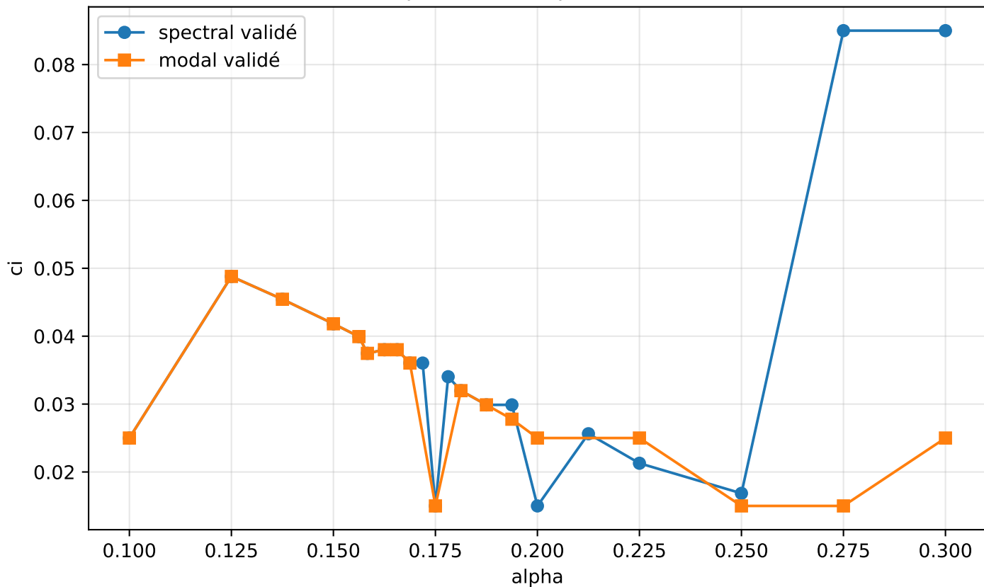
Supersonic ci(alpha), M=1.5
