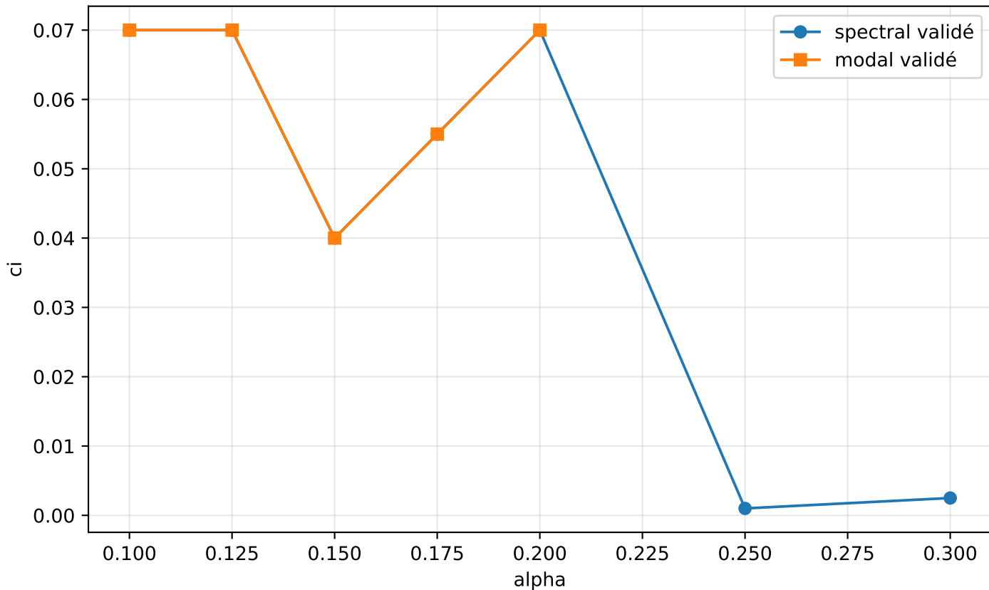
Supersonic c_i(\alpha) , M=1.1
