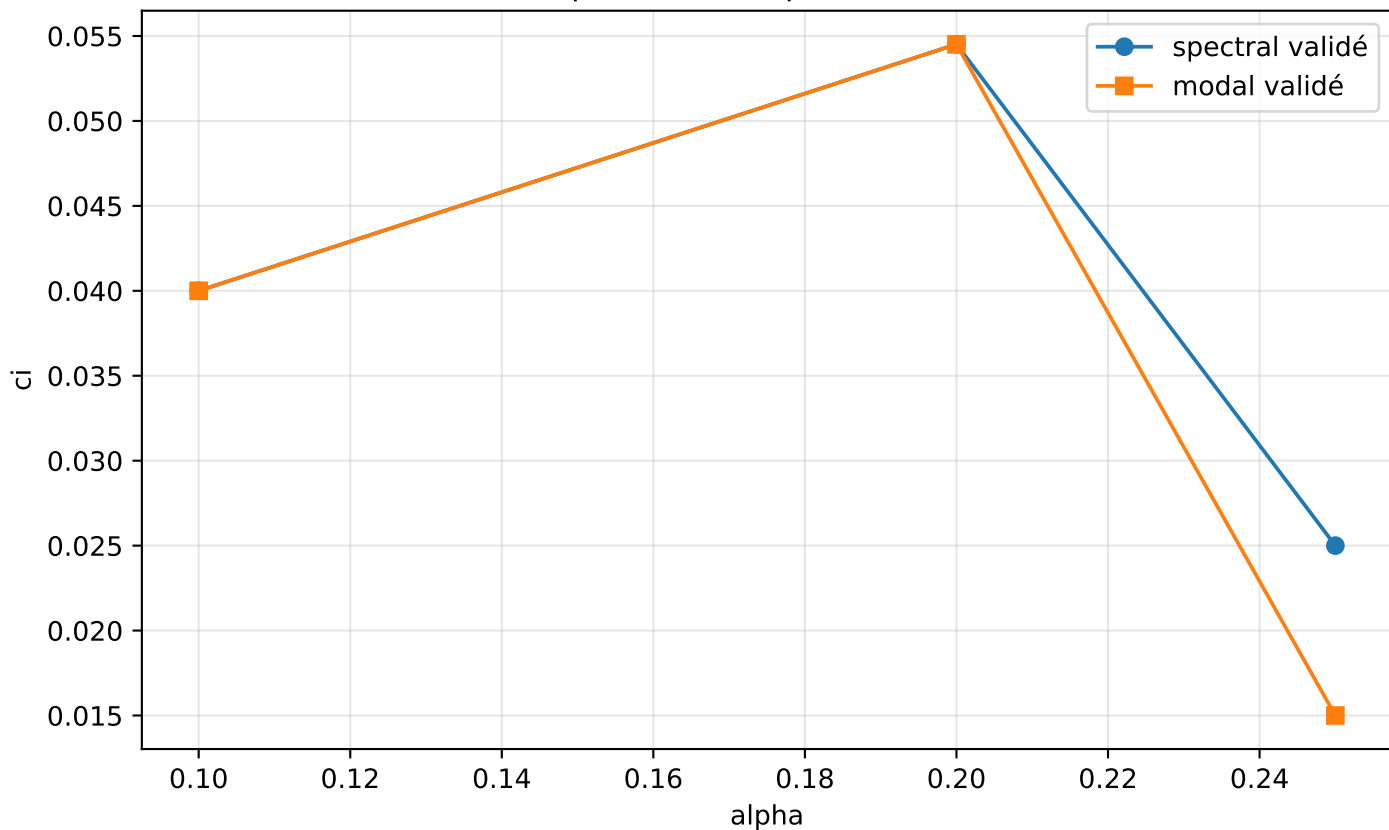
Supersonic c_i(\alpha) , M=1.25
