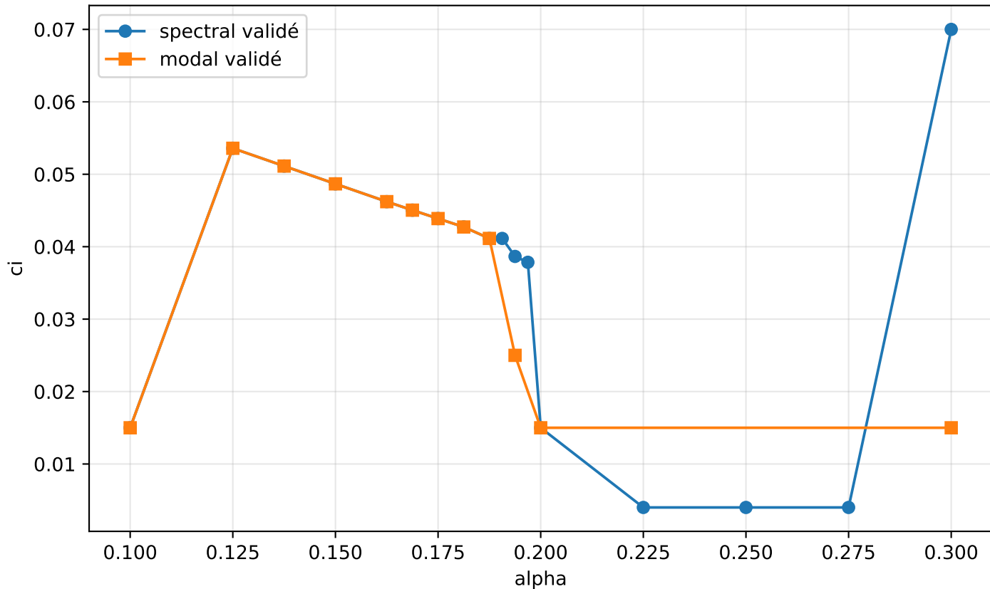
Supersonic c_i(\alpha) , M=1.4
