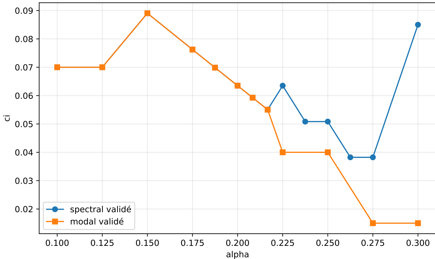
Supersonic c_i(\alpha) , M=1.2
