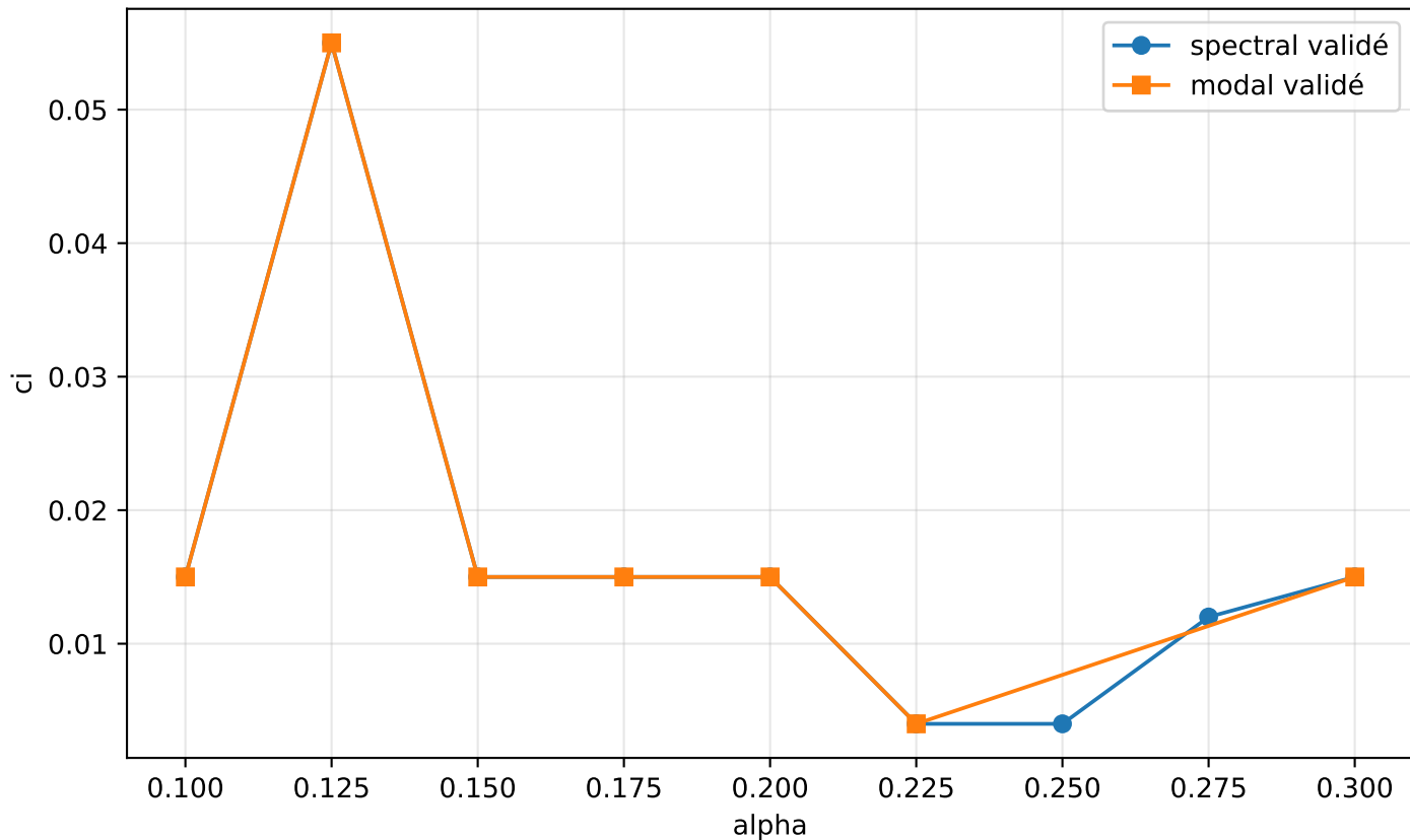
Supersonic ci(alpha), M=1.6
