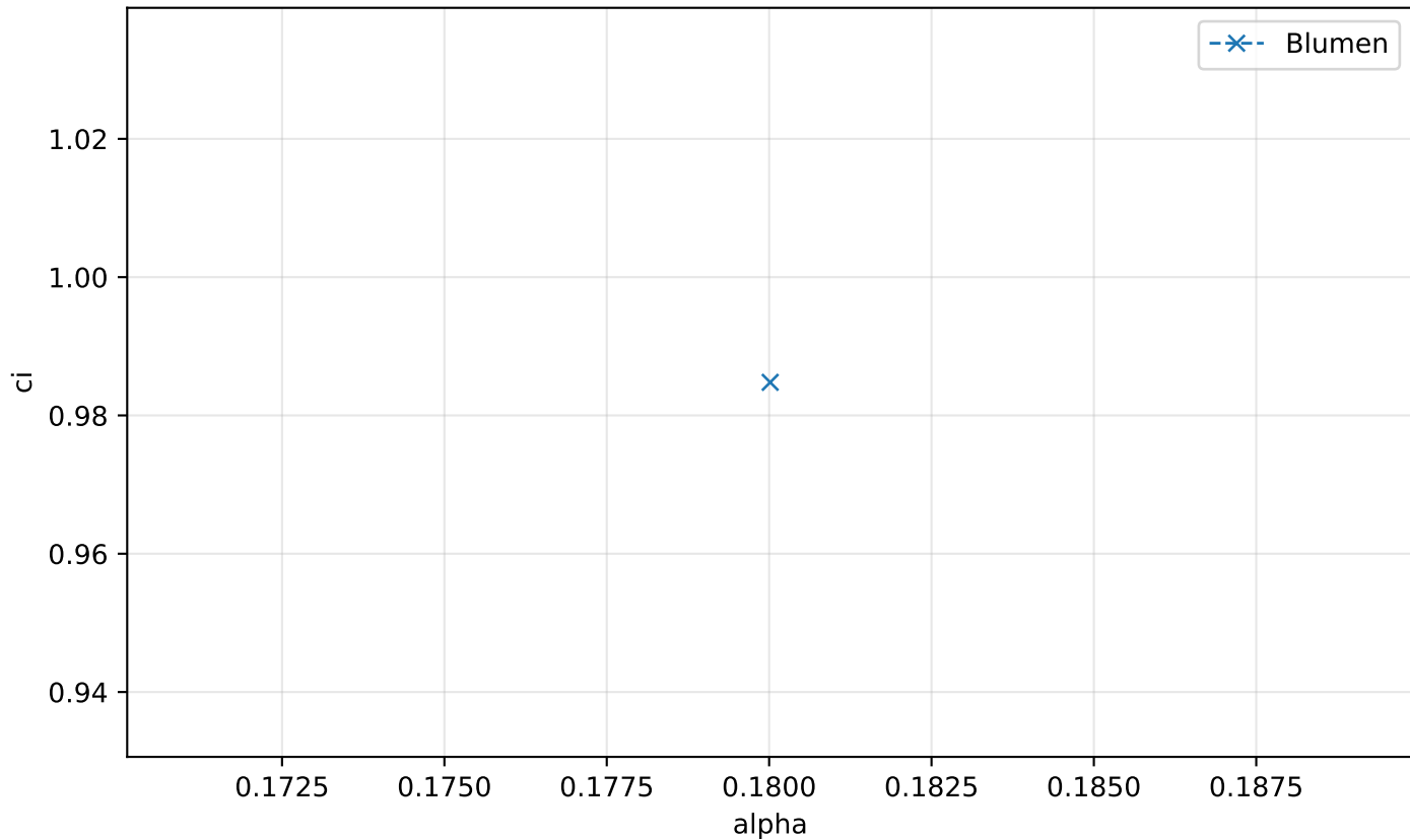
Supersonic c_i(\alpha) , M=0.180017
