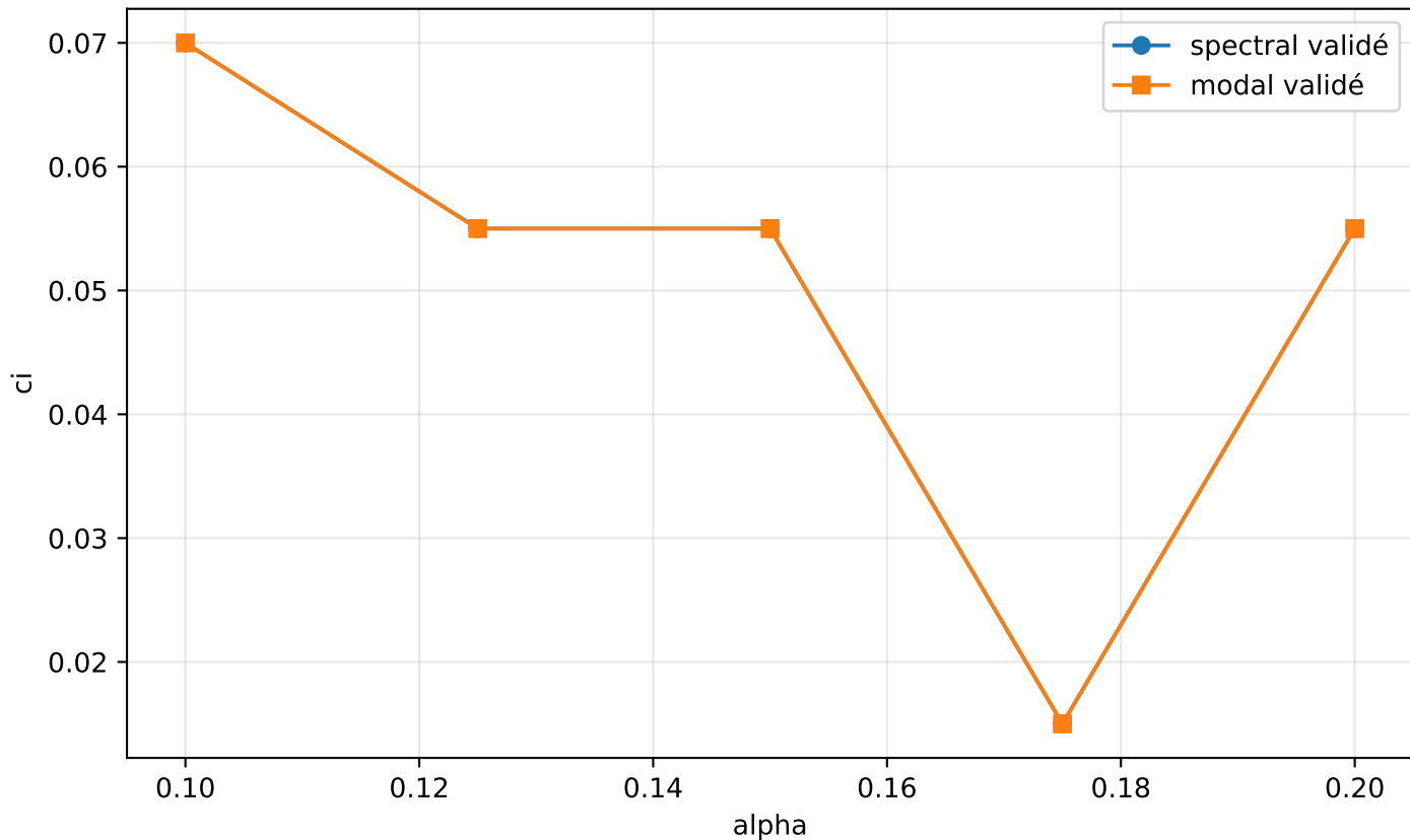
Supersonic c_i(\alpha) , M=1
