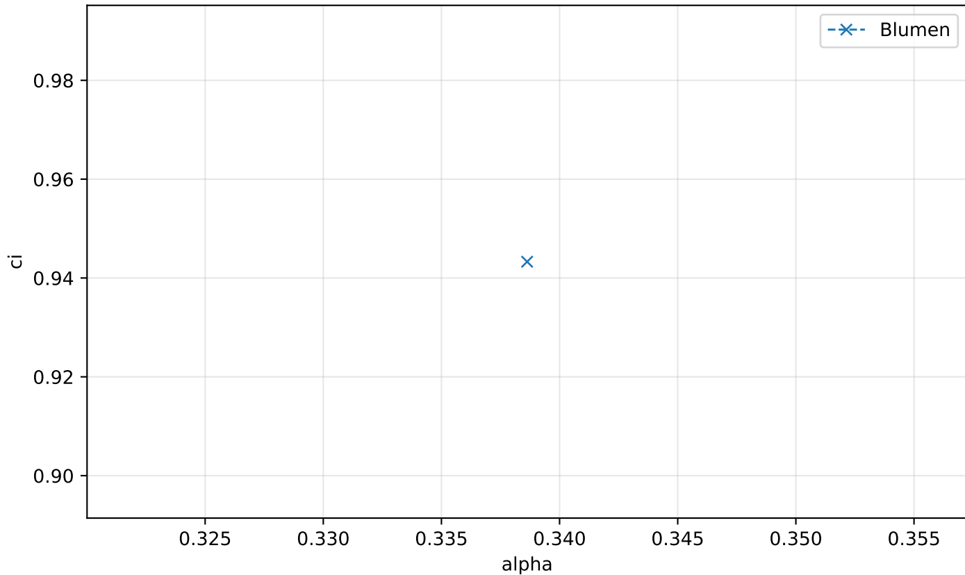
Supersonic c_i(\alpha) , M=0.338627
