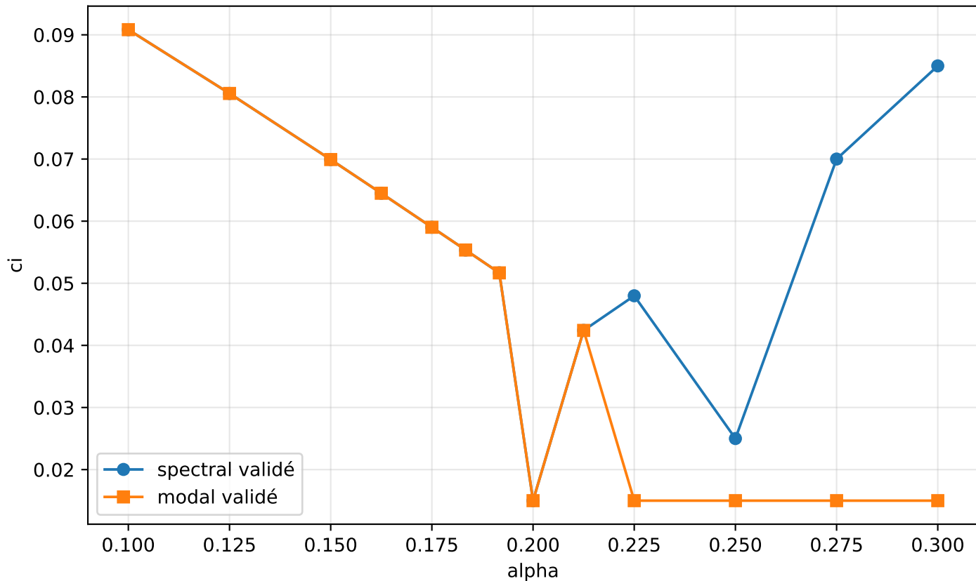
Supersonic c_i(\alpha) , M=1.3
