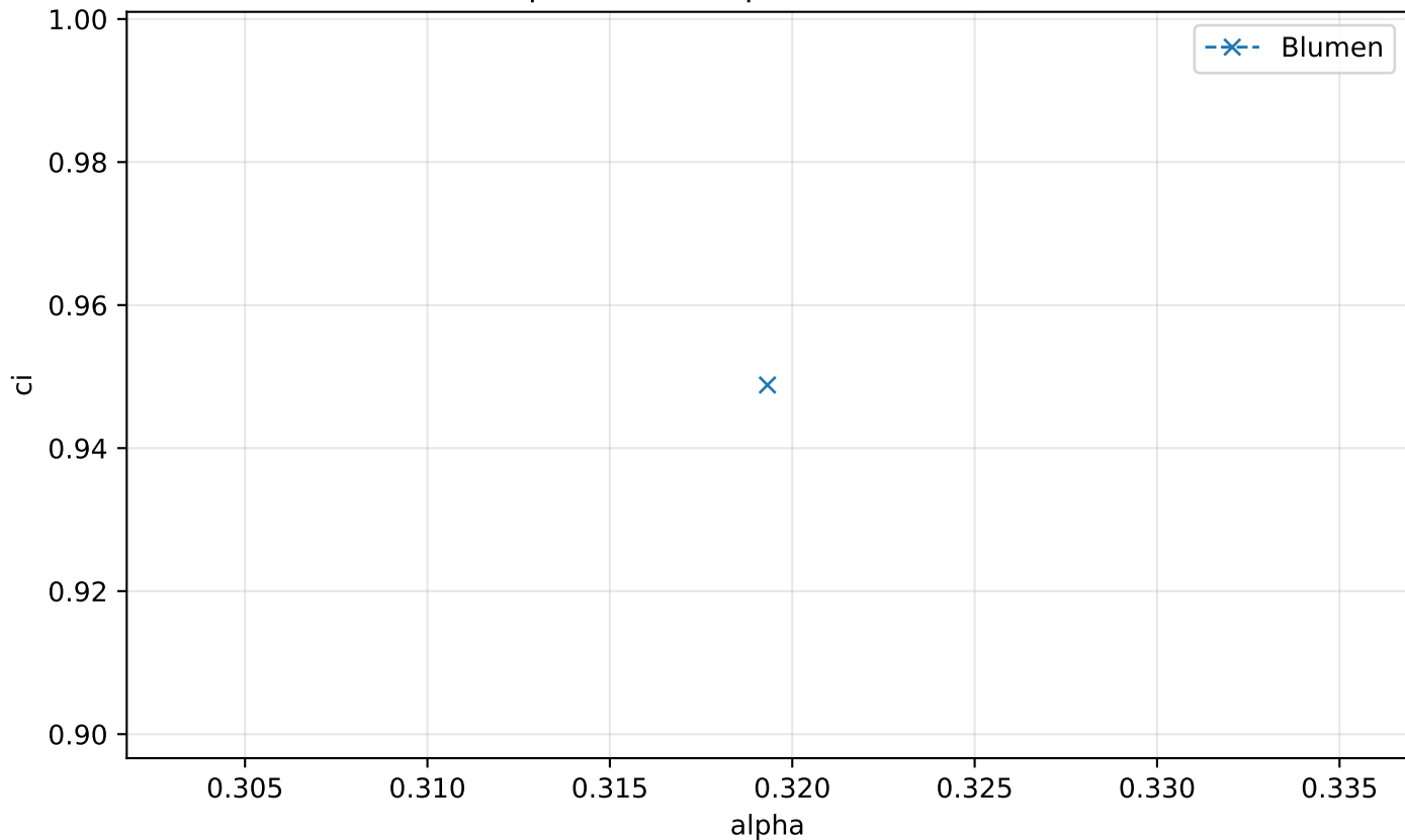
Supersonic c_i(\alpha) , M=0.319321
