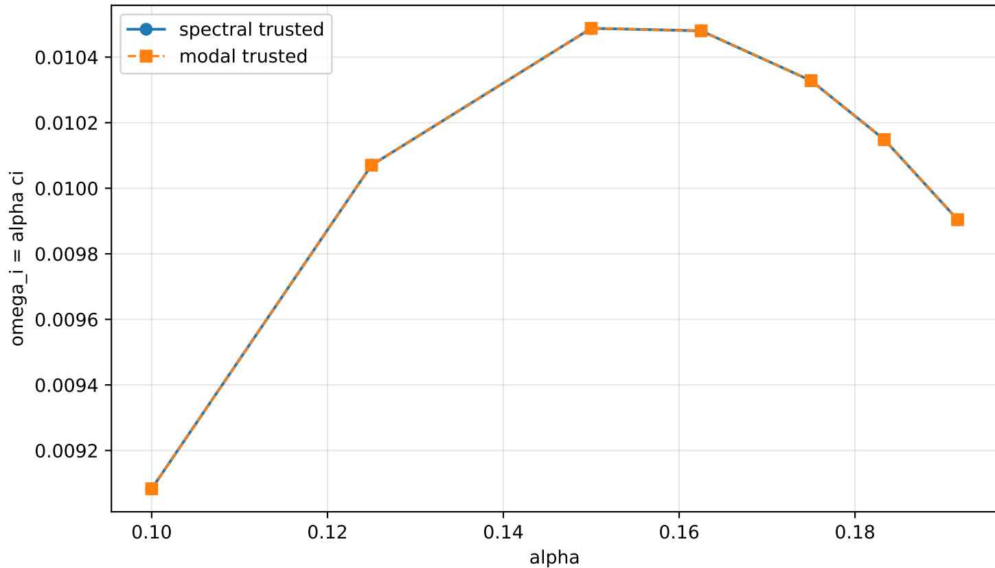
Curated strict \omega_i = \alpha c_i(\alpha) , M=1.3
