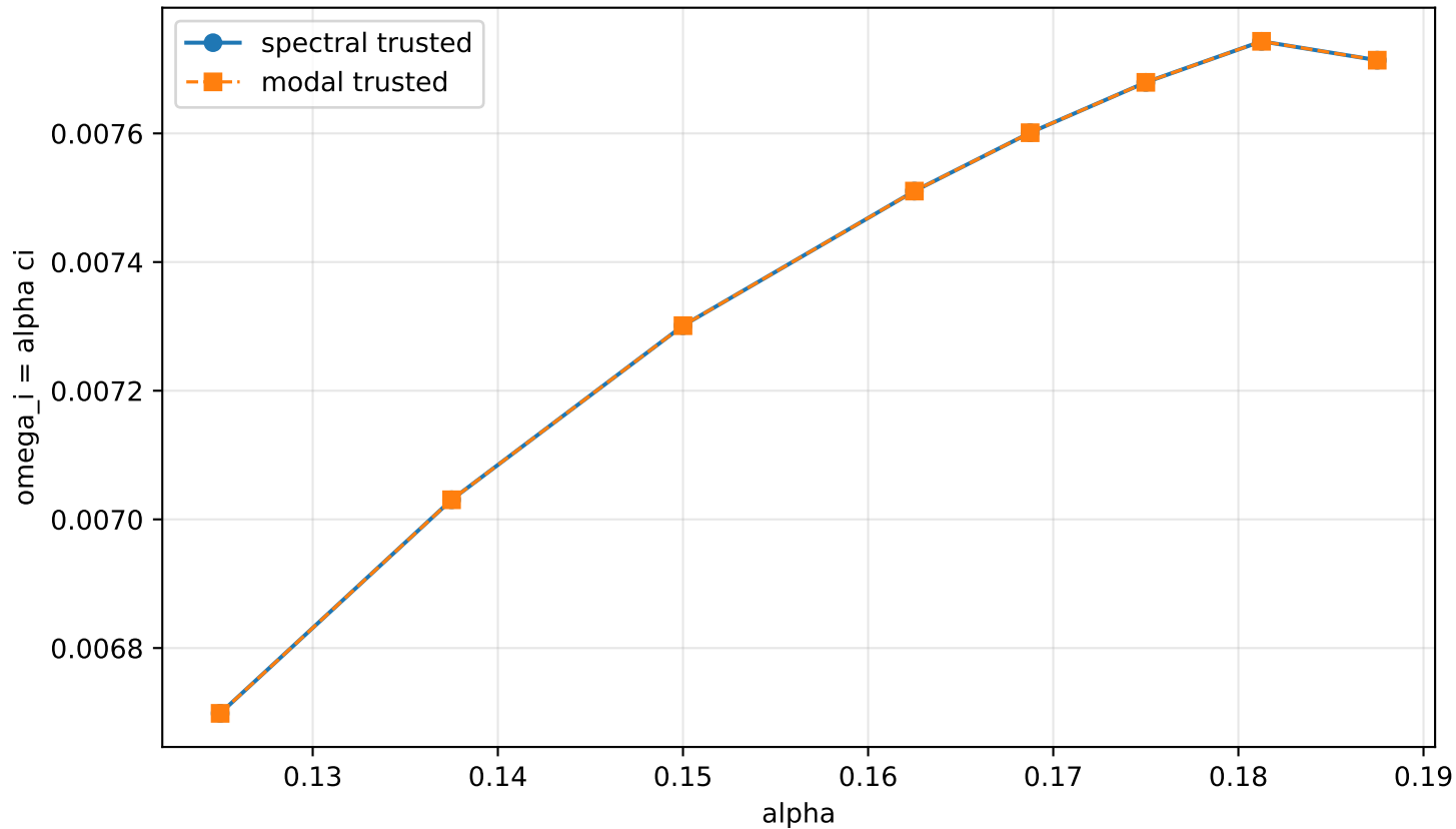
Curated strict \omega_i = \alpha \text{ci}(\alpha) , M=1.4
