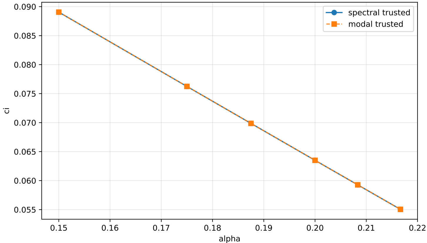
Curated strict ci(alpha), M=1.2
