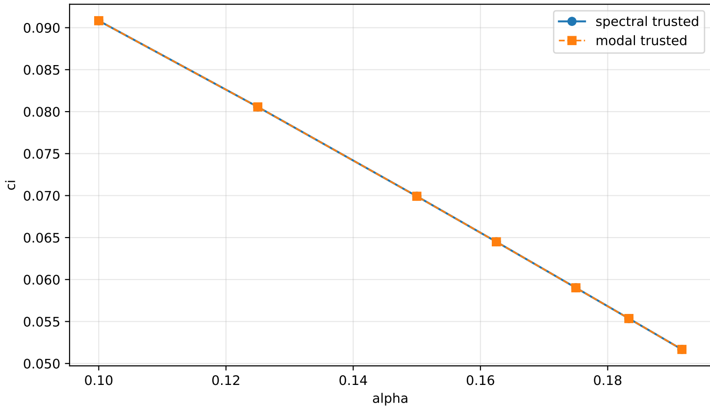
Curated strict ci(alpha), M=1.3
