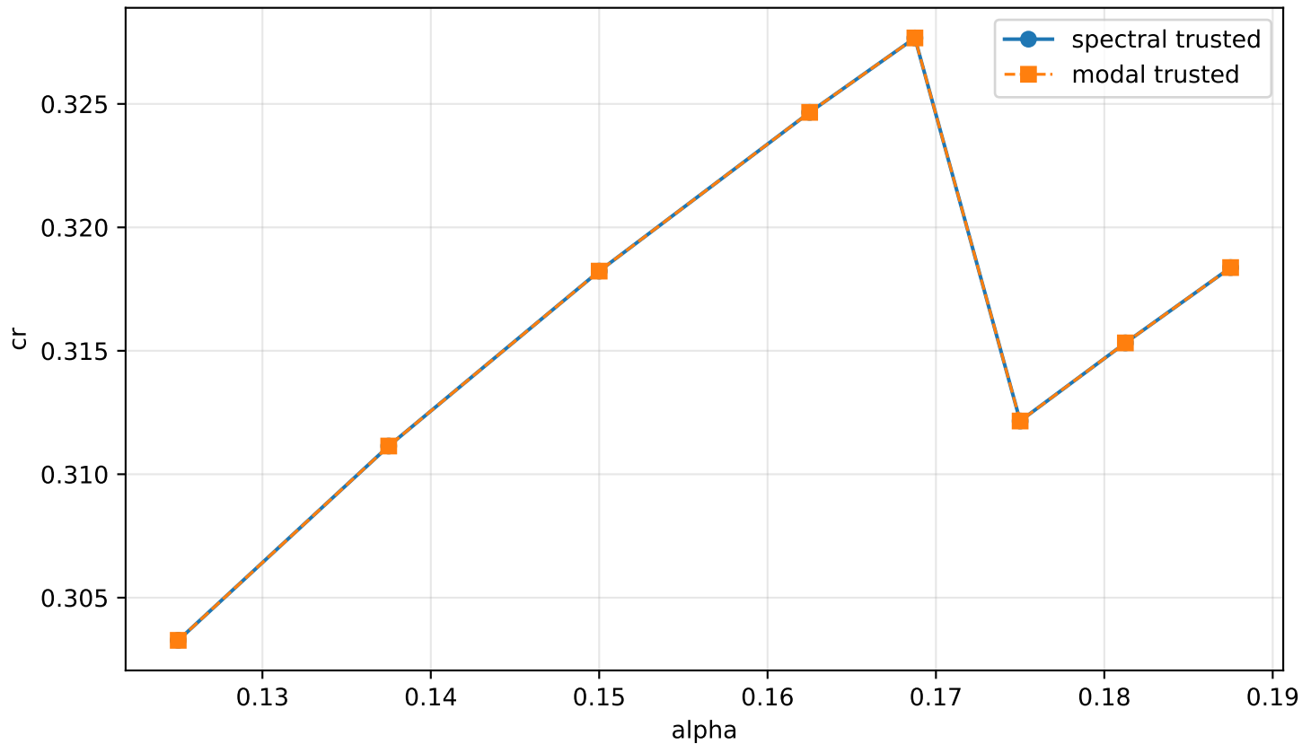
Curated strict \text{cr}(\alpha) , M=1.4
