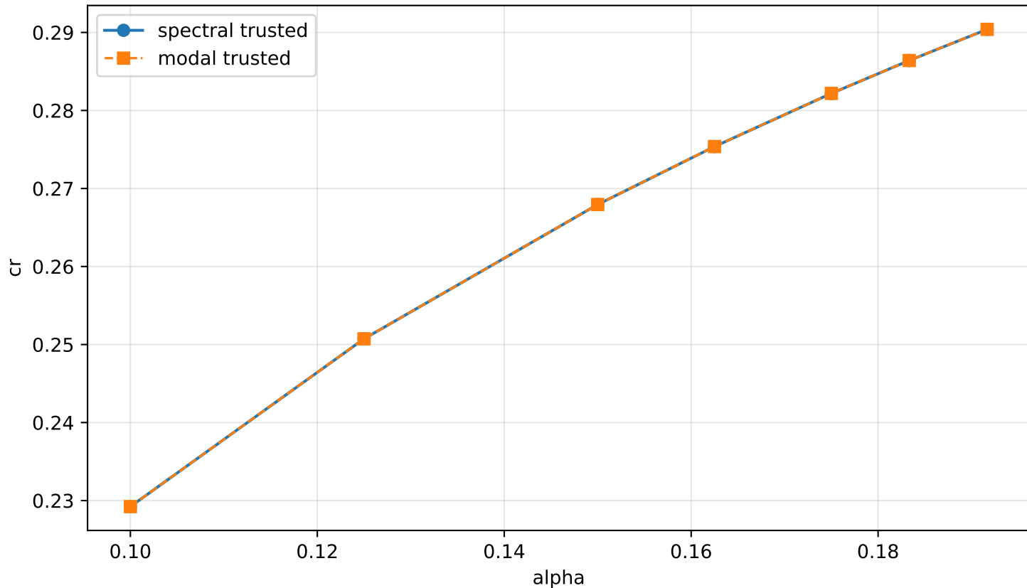
Curated strict cr( \alpha ), M=1.3
