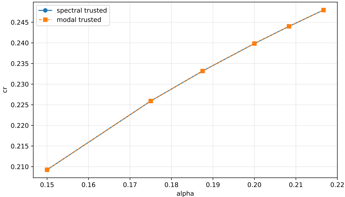
Curated strict cr(\alpha) , M=1.2
