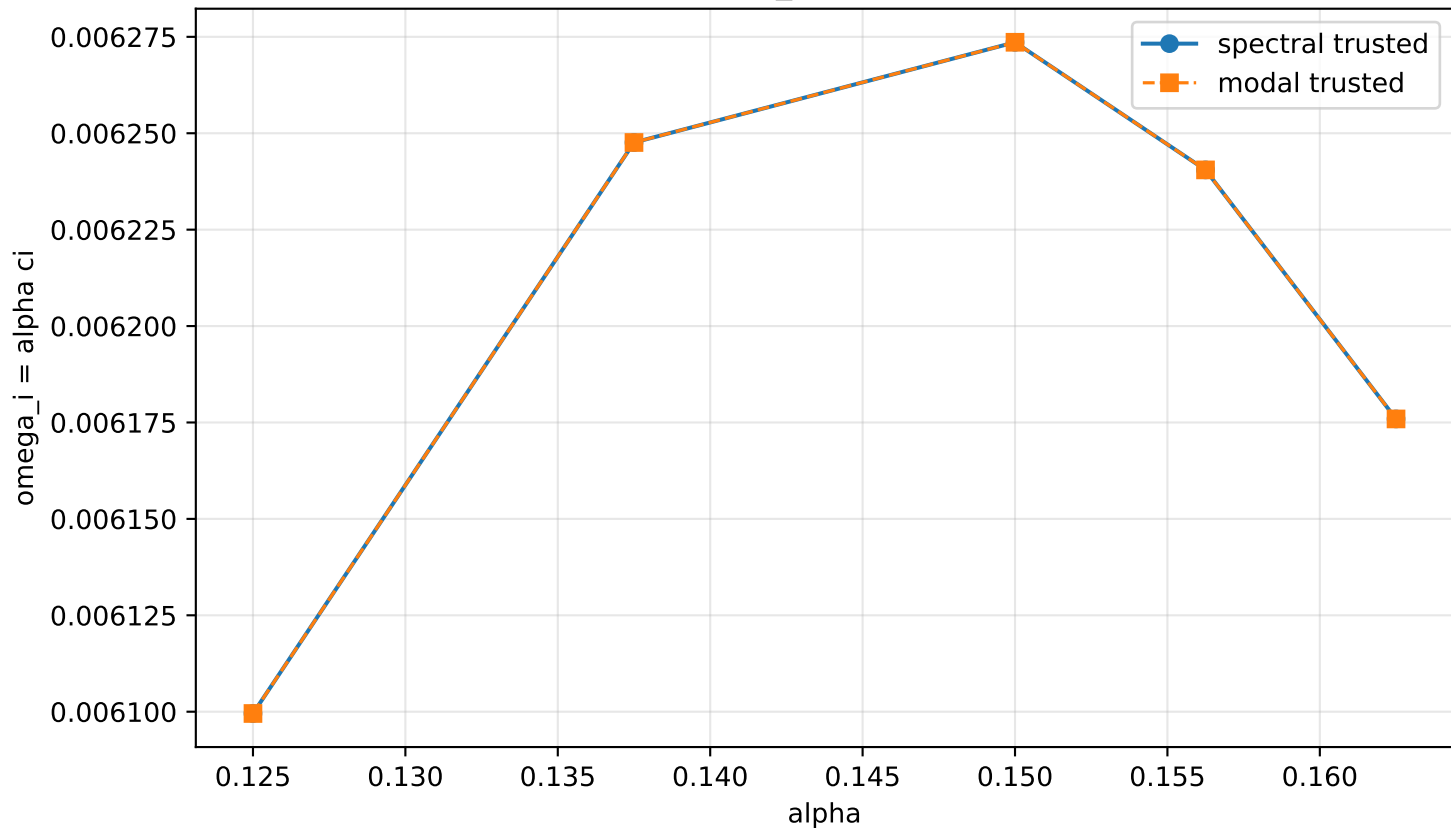
Curated strict \omega_i = \alpha \text{ci}(\alpha) , M=1.5
