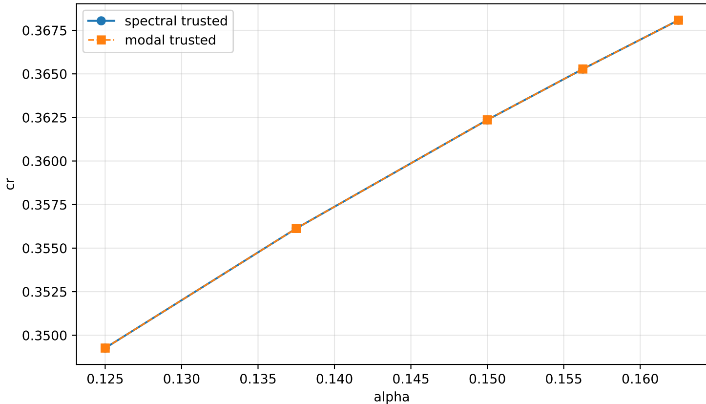
Curated strict cr(alpha), M=1.5
