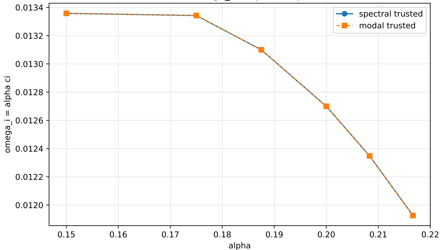
Curated strict \omega_i = \alpha c_i(\alpha) , M=1.2
