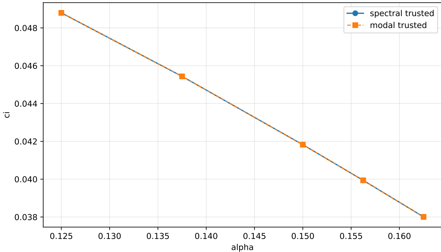
Curated strict ci(alpha), M=1.5
