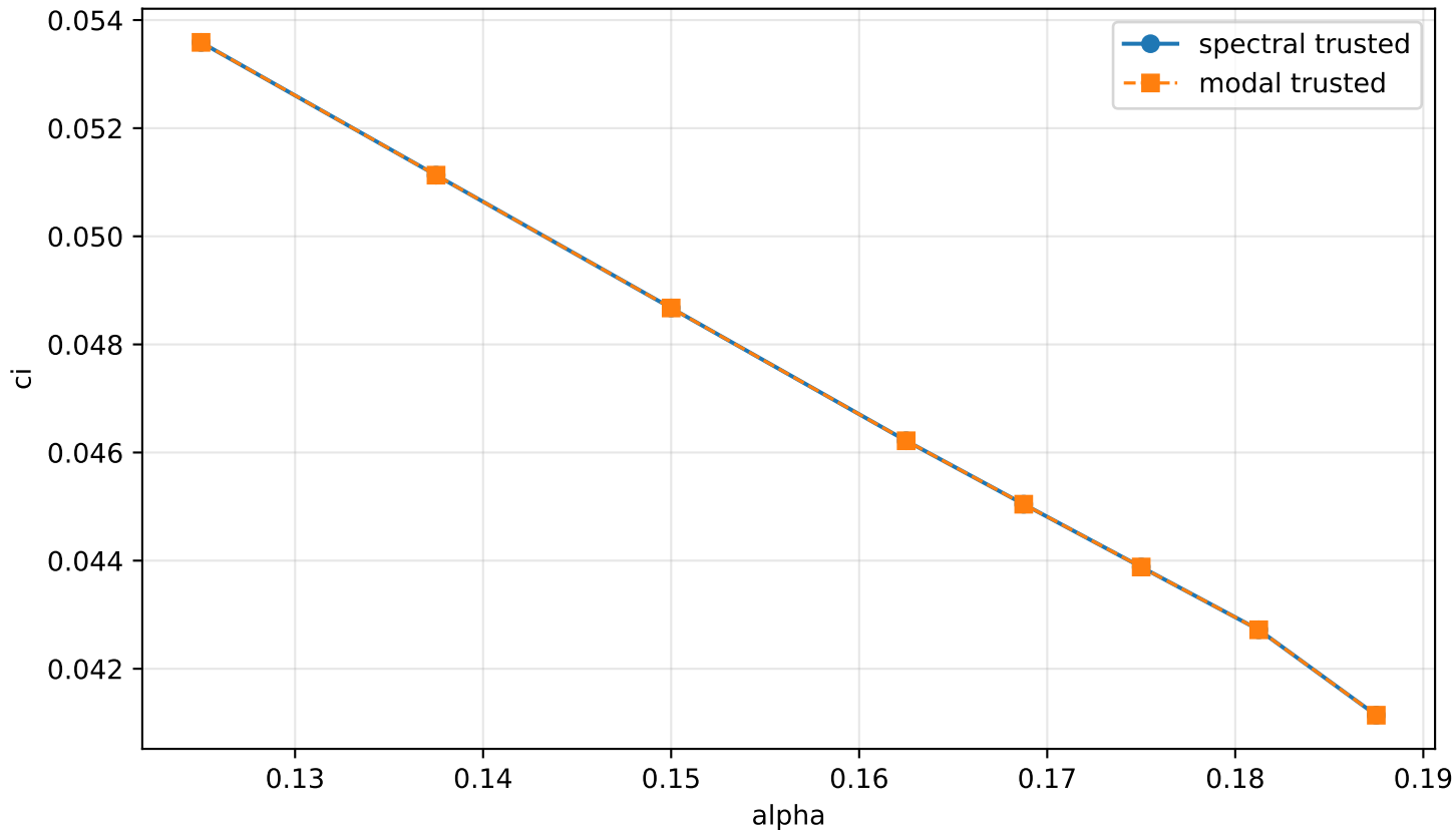
Curated strict ci(alpha), M=1.4
