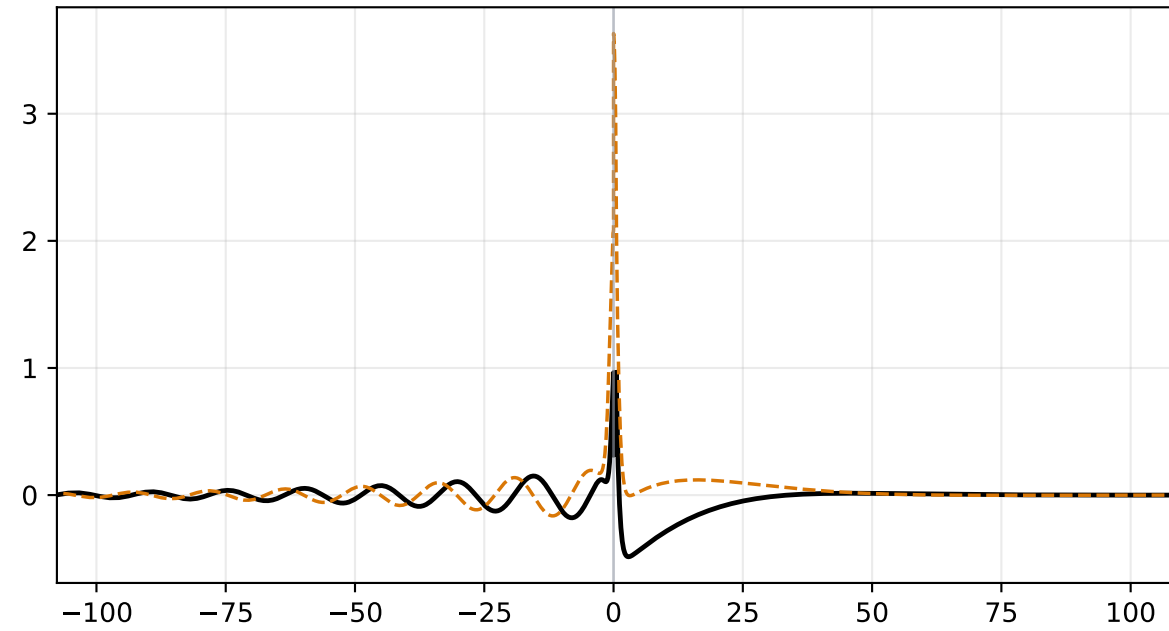
Pressure Perturbation \hat{p}
