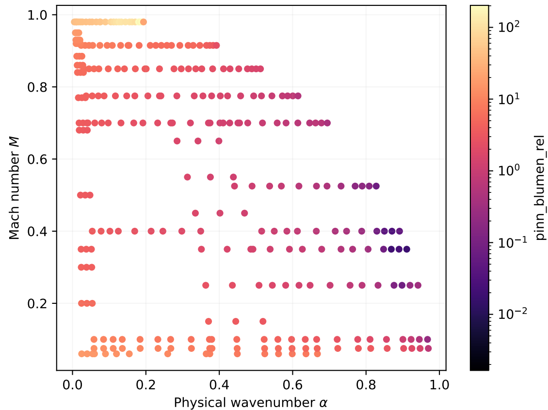
(c) Direct PINN vs Blumen: stabilized relative error
