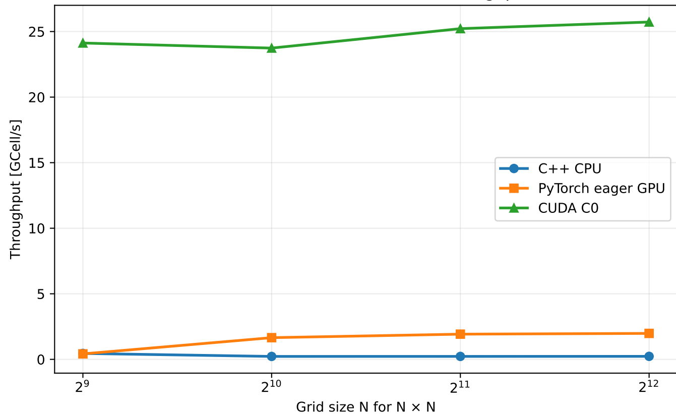
Advection-diffusion stencil — throughput
