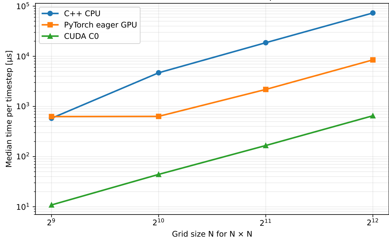
Advection-diffusion stencil — compute time
