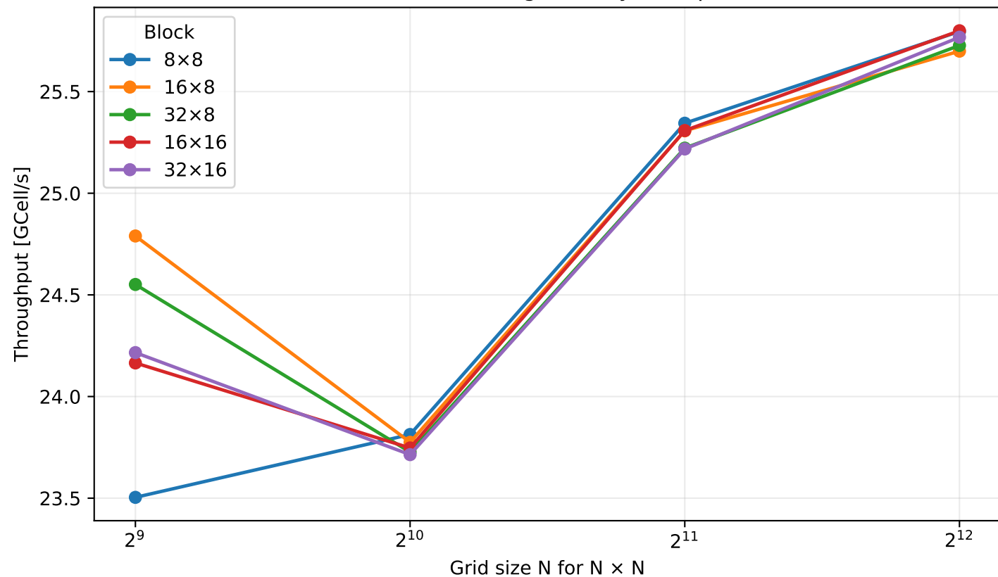
CUDA block-geometry sweep
