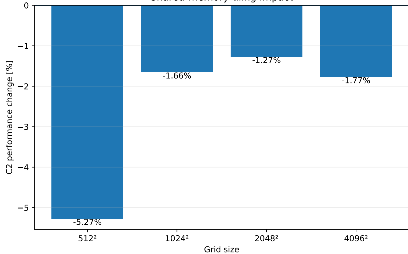
Shared-memory tiling impact
