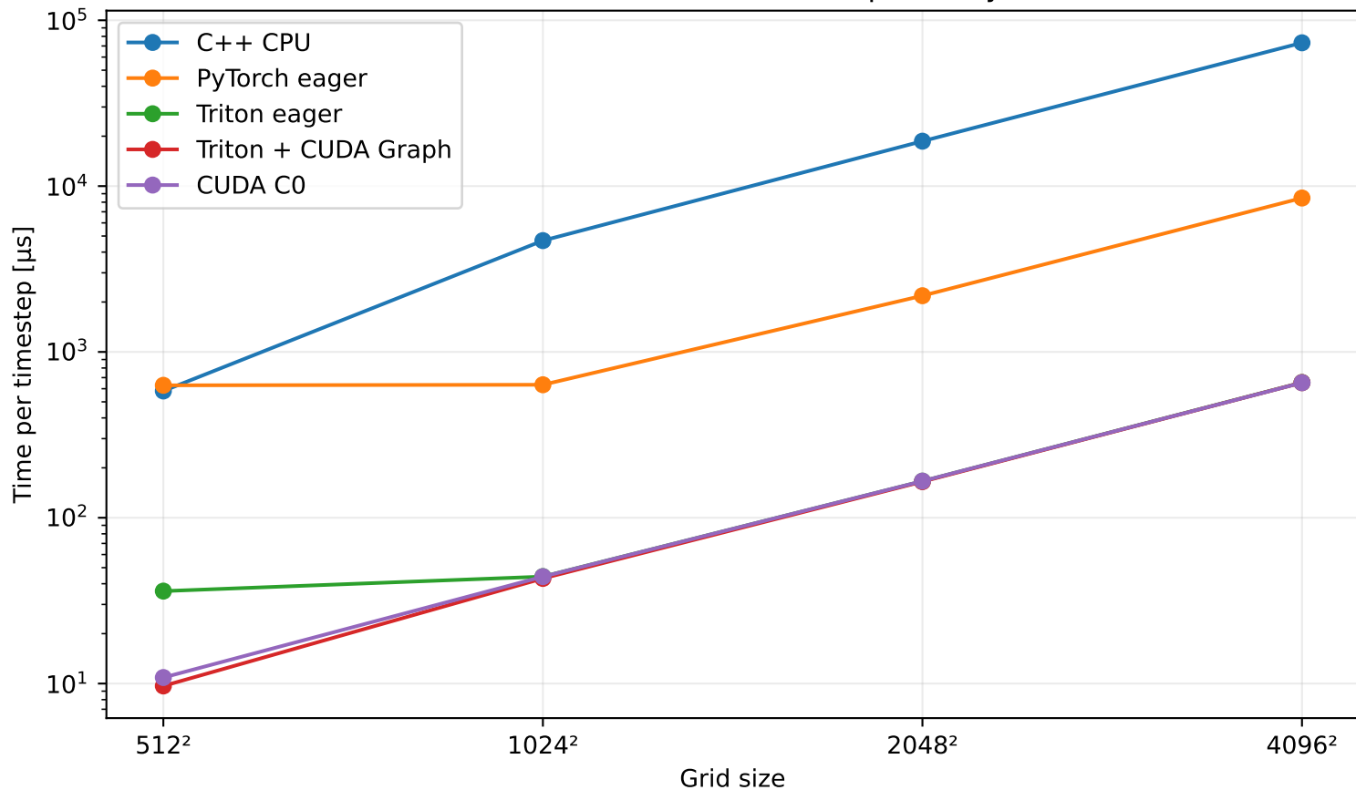
Advection-diffusion timestep latency
