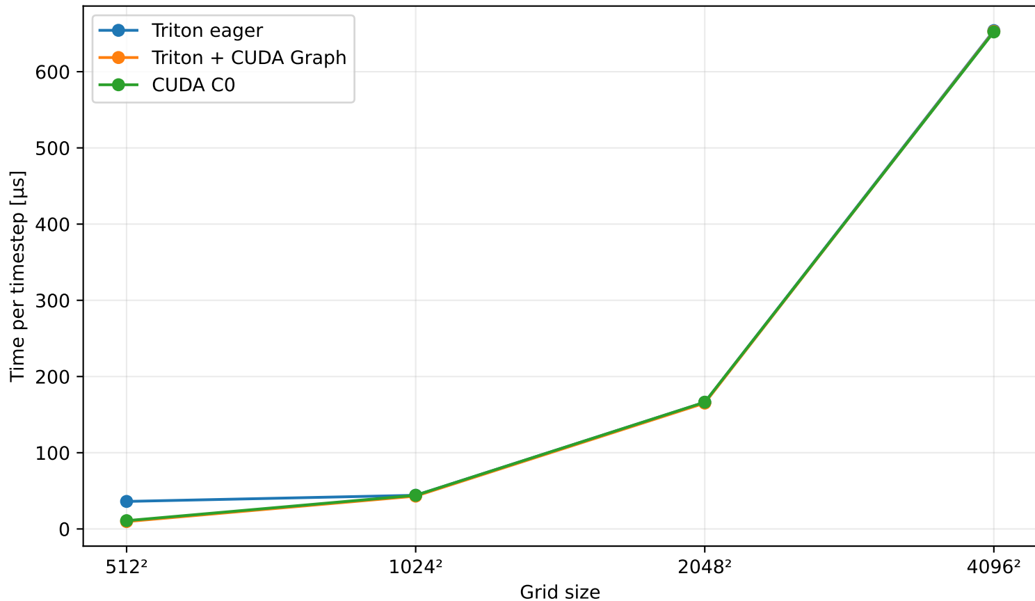
Triton dispatch overhead and CUDA Graph replay
