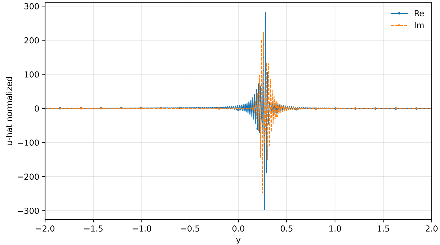
Zoom on \hat{u} | rank=4, \alpha=0.200 , M=1.200 , c=0.26153+i0.03650
