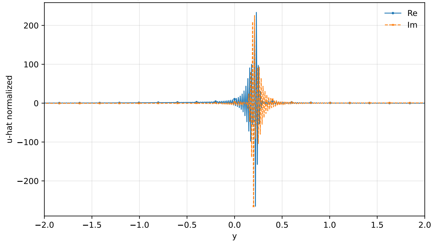
Zoom on \hat{u} | rank=5, \alpha=0.200 , M=1.200 , c=0.20840+i0.03628
