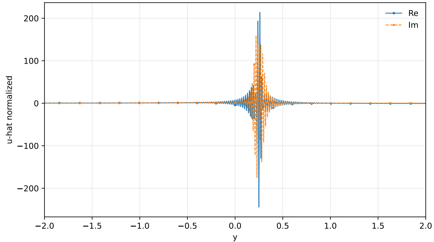
Zoom on \hat{u} | rank=2, \alpha=0.200 , M=1.200 , c=0.24375+i0.03804
