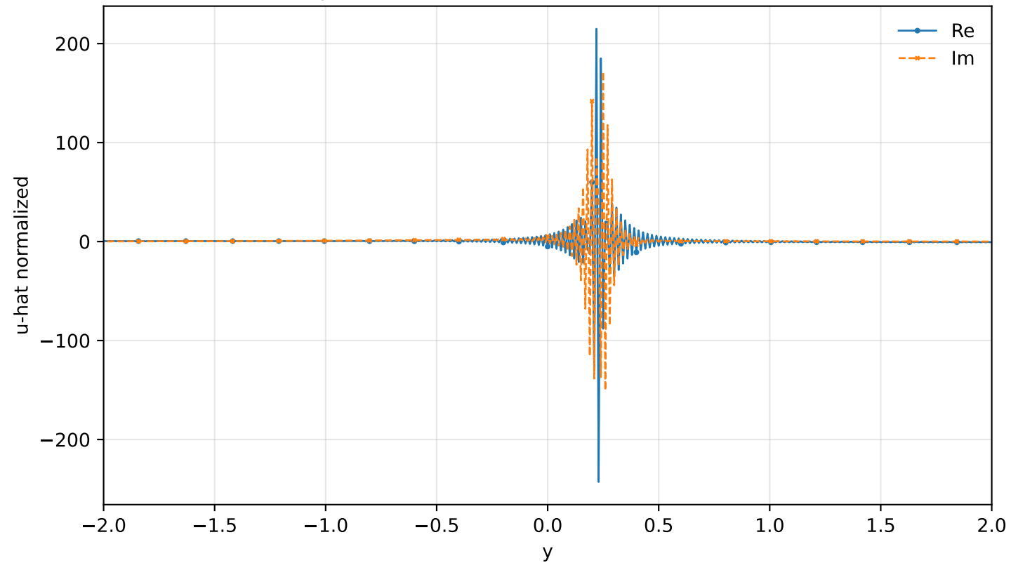
Zoom on \hat{u} | rank=3, \alpha=0.200 , M=1.200 , c=0.22602+i0.03777
