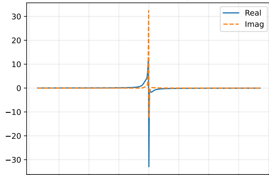
Streamwise Velocity \hat{u}
