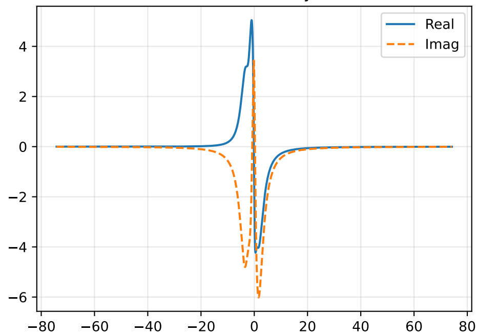
Vertical Velocity \hat{v}
