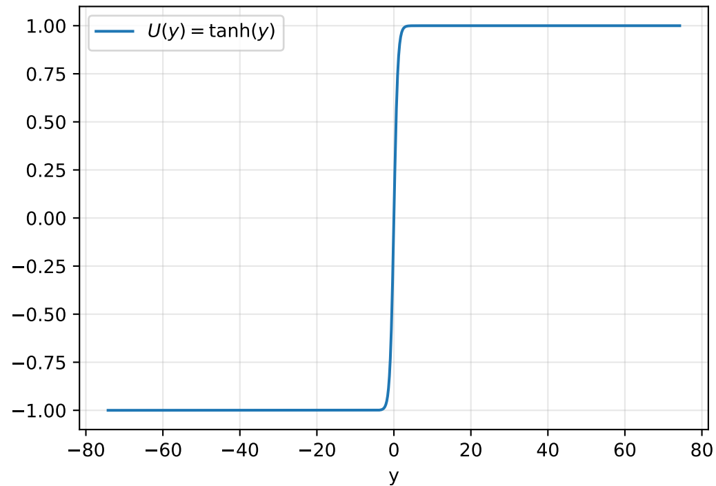
c_i^{PINN} = 0.87808 , c_i^{ref} = 0.91465
