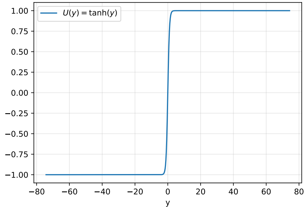
c_i^{PINN} = 0.82096 , c_i^{ref} = 0.83643
